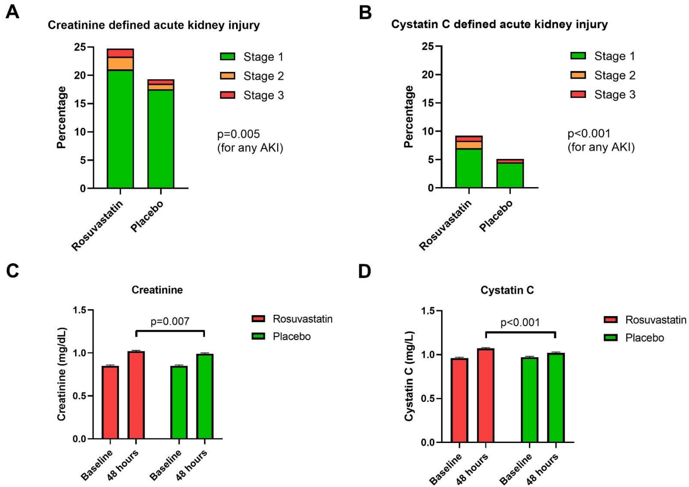
Figure 1: Effect of allocation to rosuvastatin on creatinine-defined and cystatin C-defined AKI, and on post-operative creatinine and cystatin C levels
