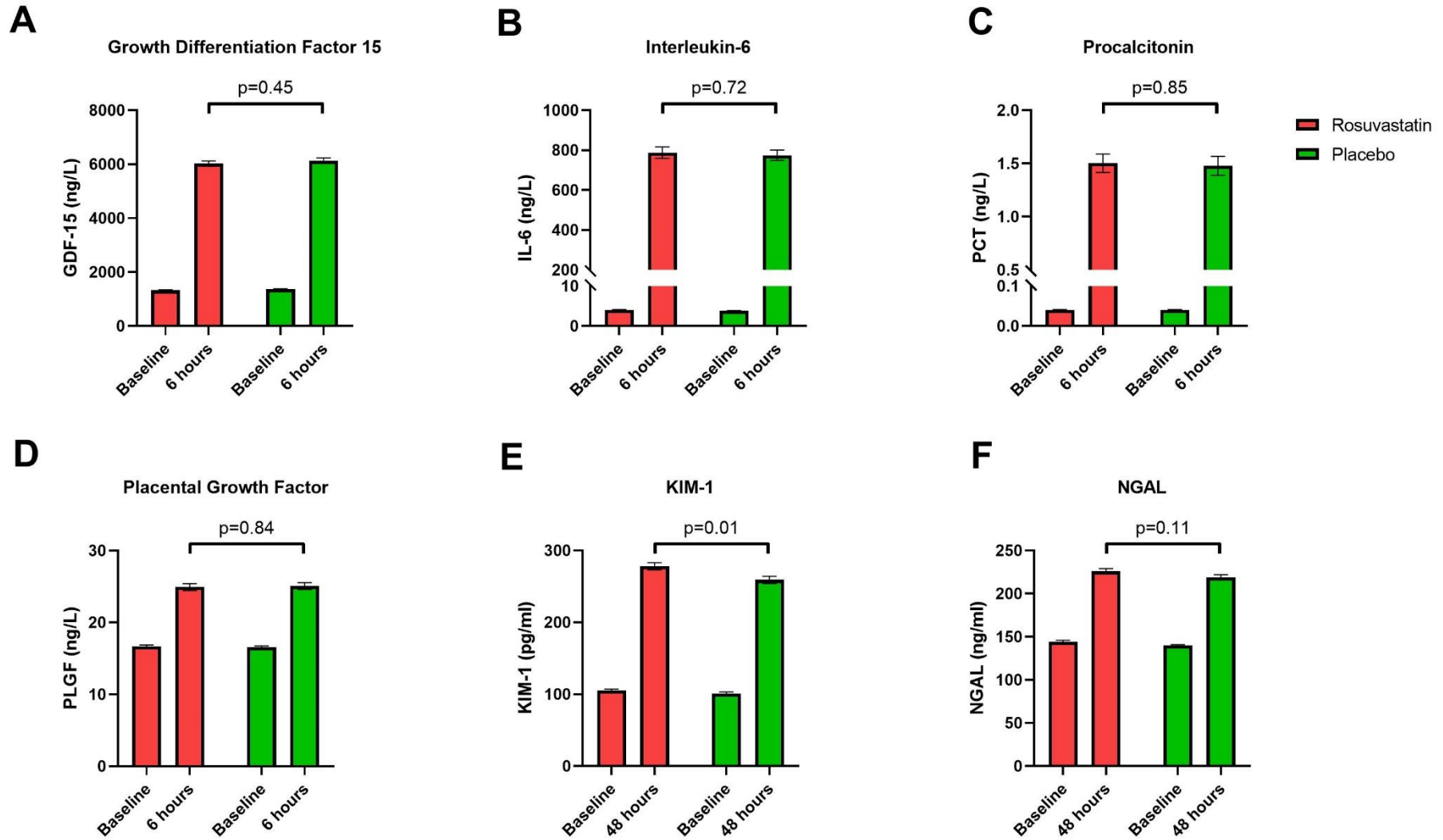
Figure 3: Effect of allocation to rosuvastatin on postoperative concentrations of biomarkers of inflammation and renal injury
