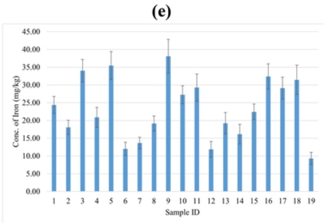
Figure 2. Mean concentration of heavy metals: (a) Lead (Pb), (b) Cadmium (Cd), (c) Chromium (Cr), (d) Copper (Cu), (e) Iron (Fe).
