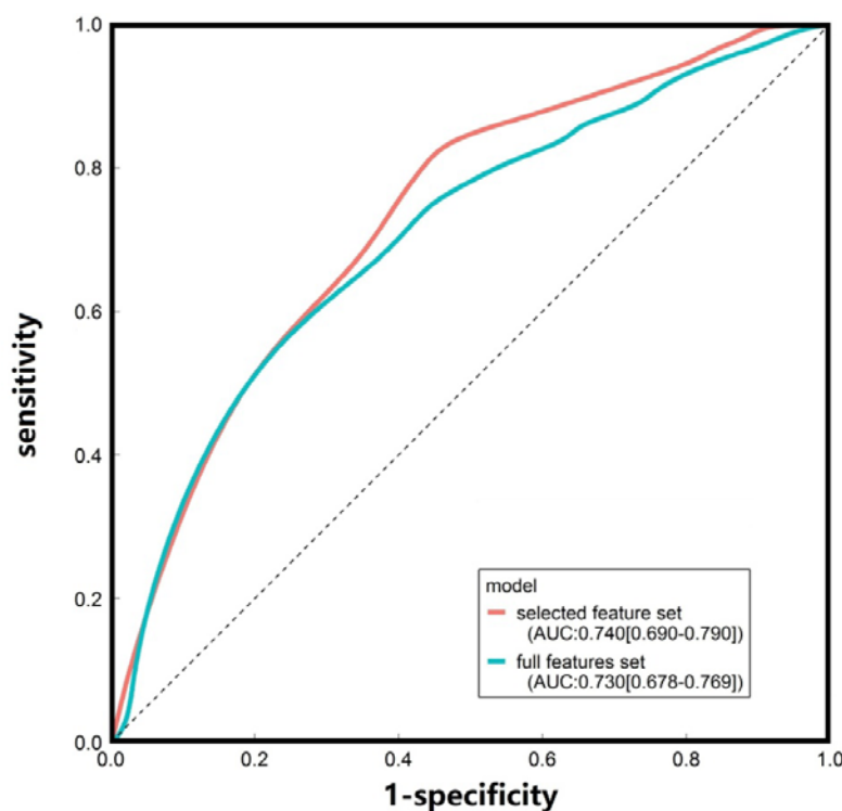
Figure 2. ROC curves of the SVM models constructed based on the median gene expression levels in different tissue-age groups
