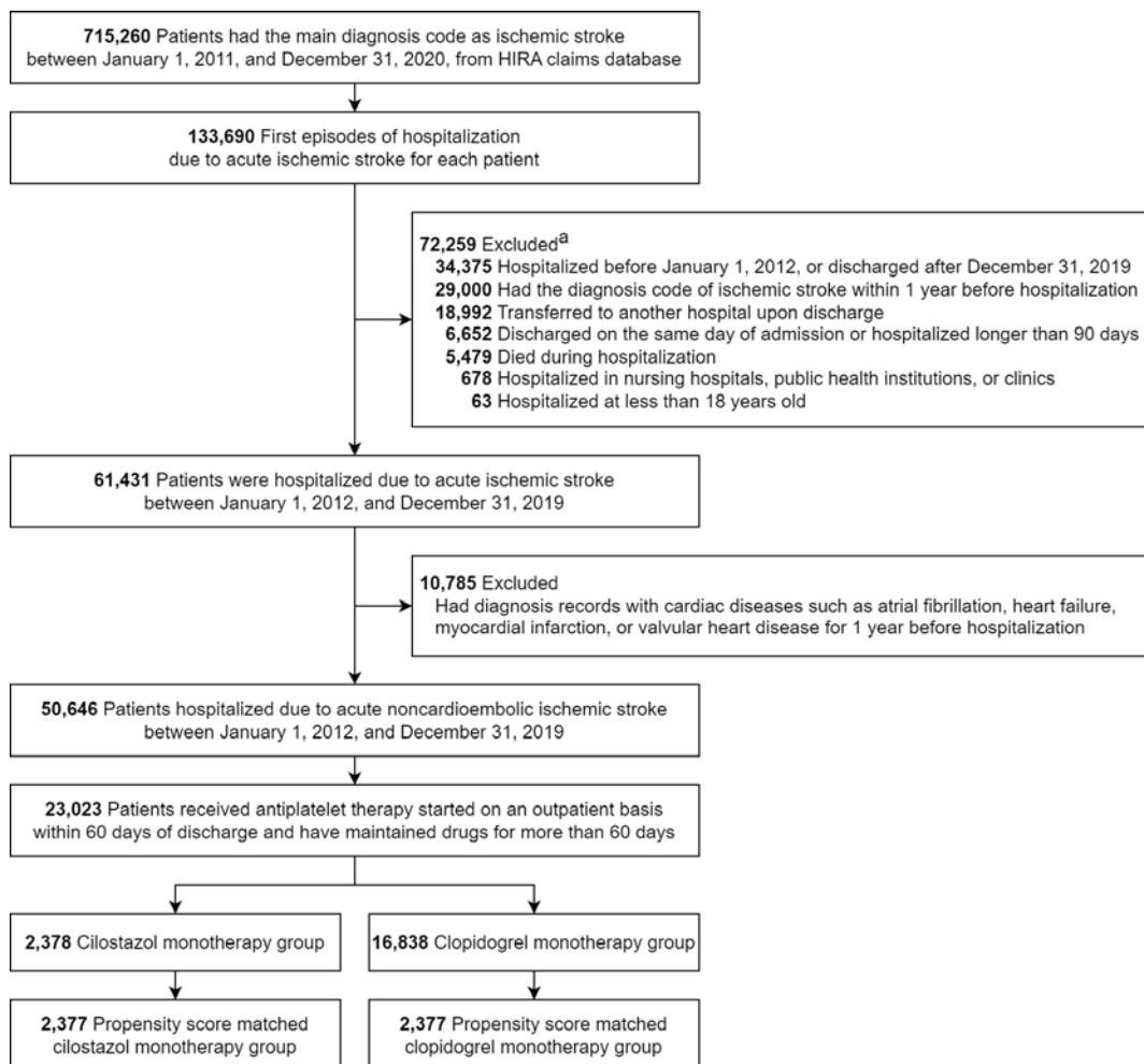
Figure 1. Study flowchart
