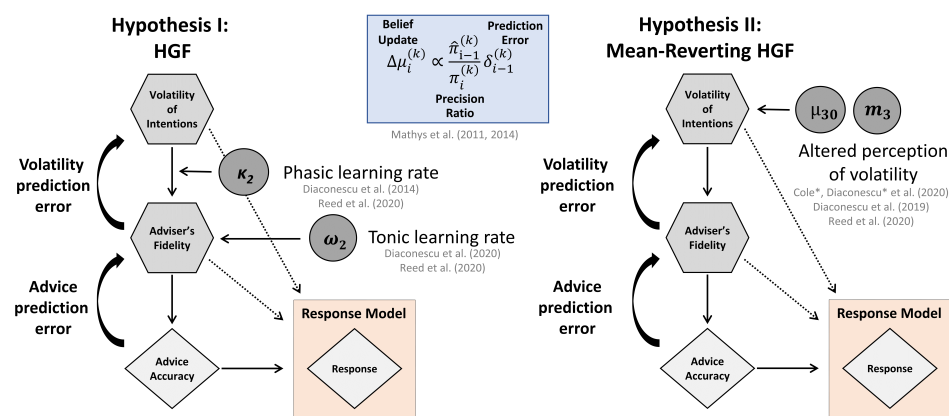
Figure 3: Model space. Left: Standard 3-level Hierarchical Gaussian Filter (HGF) (Mathys et al., 2011, 2014) Right: Mean-reverting HGF with a drift at the third level, which captures learning about the volatility of the adviser's intentions. This model expresses the notion that early psychosis may be characterised by an altered perception of environmental volatility.
