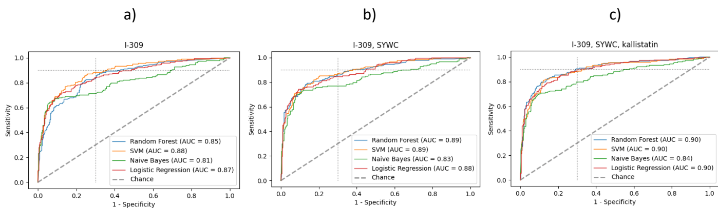
Figure 2: Receiver Operator Characteristic (ROC) curve of different machine learning algorithms with 5-fold cross validation for best performing (a) single biomarker, (b) combination of two and (c) three different biomarkers
