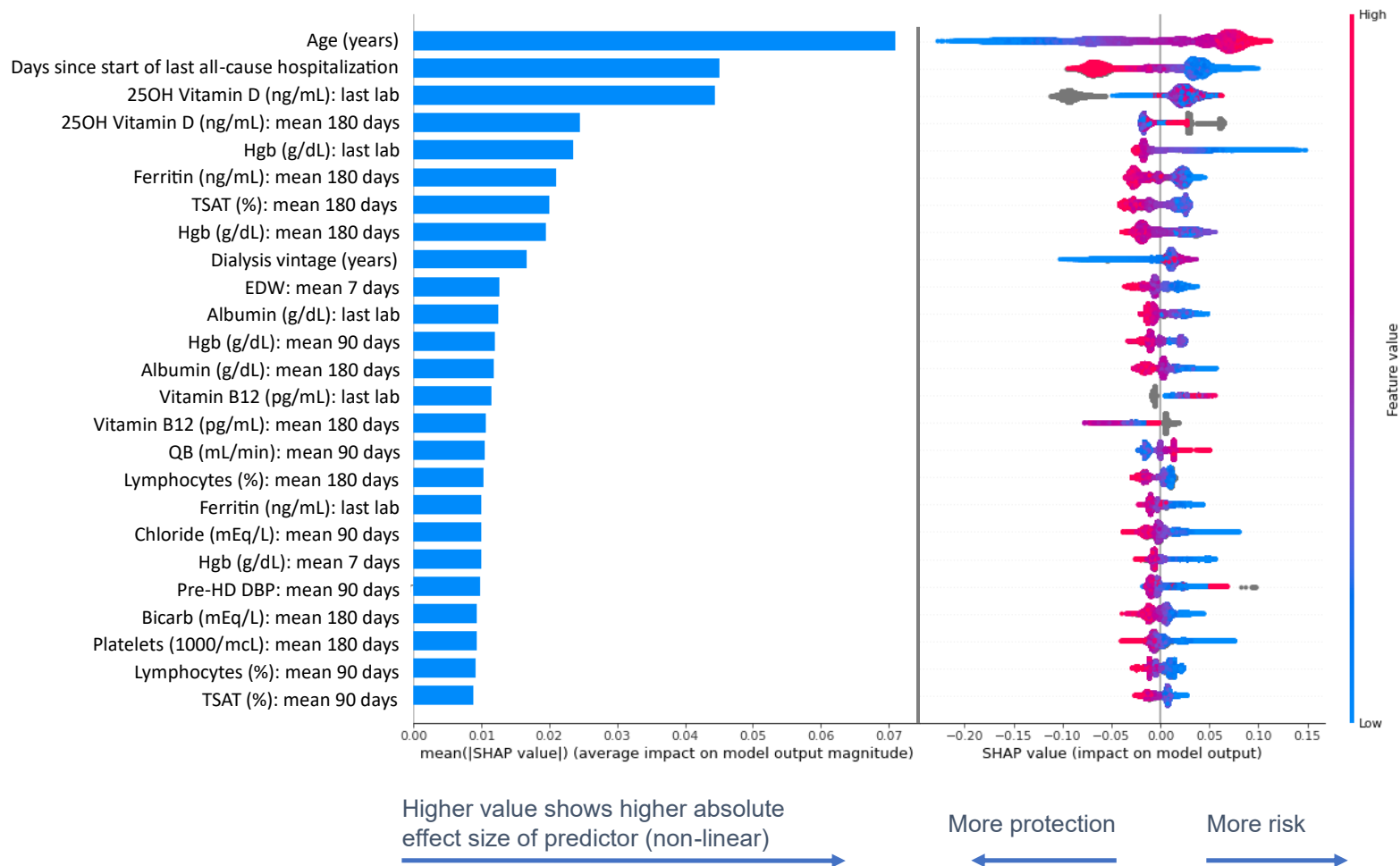
Figure 2: Top 25 predictors of 180-day GIB hospitalization in descending order. Bar plot on the left panel show the mean absolute SHAP values that estimate the average effect size of each exposure variable's contribution to predicting the outcome on the x-axis (calculated from the average absolute value for all patients). SHAP value plots in the right panels show the size and direction (more positive=higher risk or more
