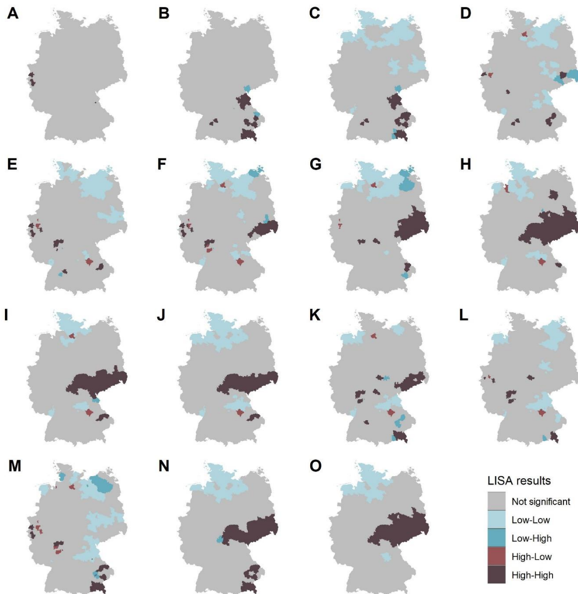
Figure 2: Local indicators of spatial autocorrelation of pandemic severity for the fifteen phases of the pandemic during 2020 and 2021 (A-O).
