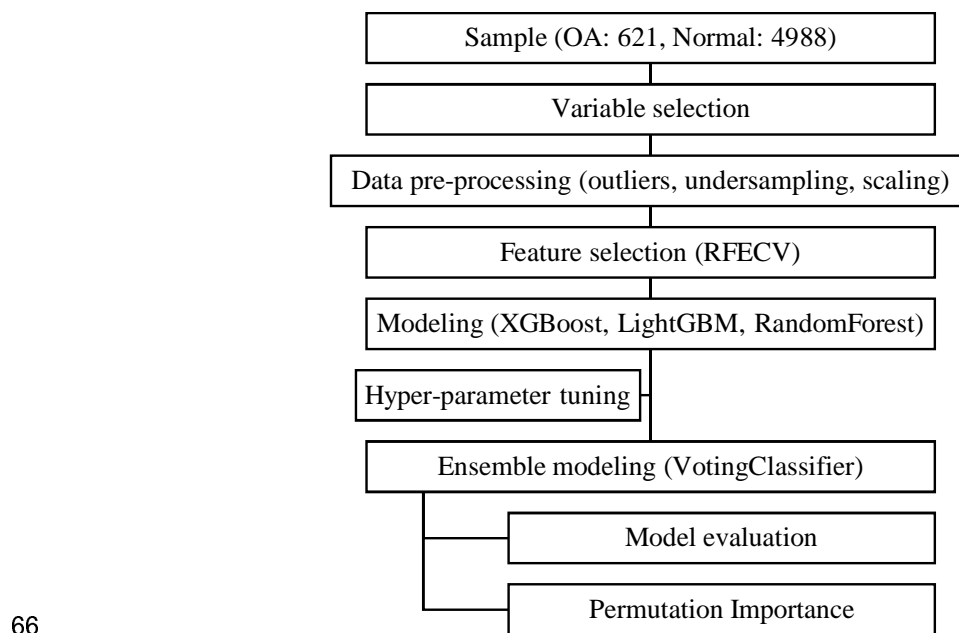
67 Figure 1. The flowchart diagram of the research process.
