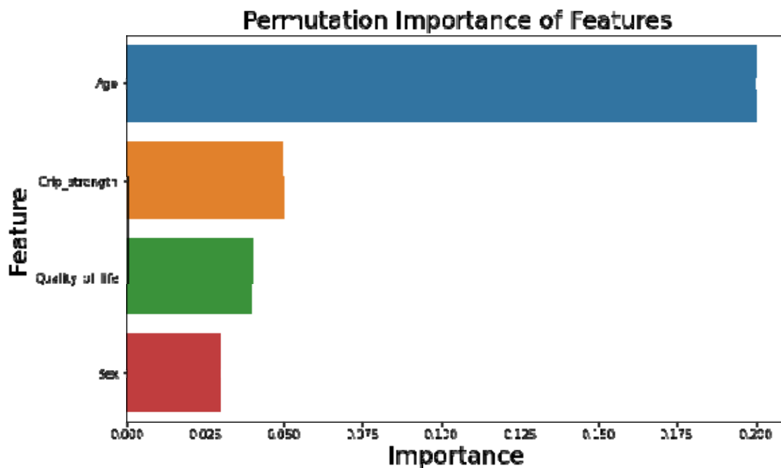
129 Figure 2. Permutation importance of features in the model
