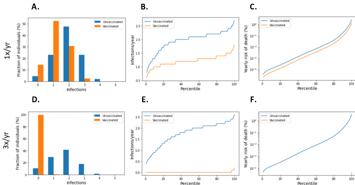
Figure 5: Three yearly boosters may prevent infection in nearly all vaccinees for a vaccine with nAb kinetics similar to post-infection. Column A shows the distribution of infection counts in a single year, which is driven by stochasticity and interindividual heterogeneity. Column B represents the average frequency of infection over a 10-year simulation, at which point interindividual heterogeneity dominates random effects. Column C shows interindividual heterogeneity in yearly risk of COVID-19 death.
