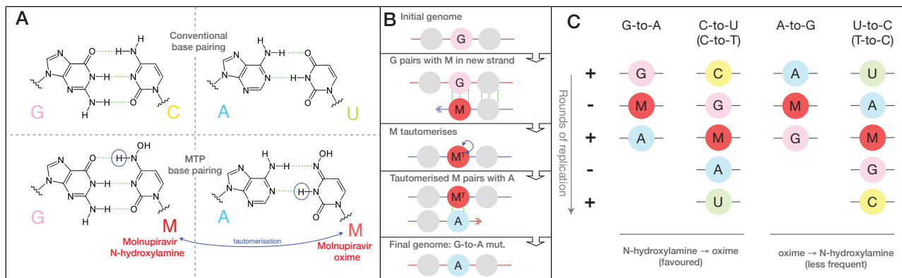
Figure 1. Molnupiravir induces mutations by acting as a nucleotide analogue with multiple tautomeric forms which pair preferentially with different nucleotides. (A) Molnupiravir triphosphate can assume multiple tautomeric forms which resemble different nucleotides. The N-hydroxylamine form resembles cytosine (C), and like cytosine can pair with guanine (G) while the oxime form more closely resembles uracil (U), and thus can pair with adenine (A). (Figure adapted in part from Malone et al. 1 ) (B) In the most common scenario, molnupiravir (M) is incorporated in the N-hydroxylamine form opposite a G nucleotide. It can then tautomerise into the oxime form, which can then pair to an A in subsequent replication, creating a G-to-A mutation. (C) Molnupiravir can result in four different mutation types. In the first column a G-to-A mutation is created by M incorporation opposite a positive-sense G, which can then pair with an A in the next positive-sense synthesis. In the second column, the positive-sense genome contains a C, which results in a G in the negative-sense genome. This G can then undergo the same G-to-A mutation, creating an negative-sense A which finally results in a U in the positive sense genome, meaning the entire process results in a C-to-U mutation. Although the biases of tautomeric forms for the free and incorporated MTP nucleotides appear to favour this directionality of mutations, with M incorporated in the N-hydroxylamine form and then transitioning to the oxime form, the reverse can also occur: this results in A-to-G and U-to-C mutations.
