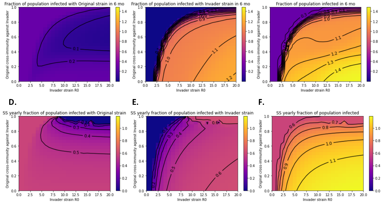
Figure 3. Short-term and long-term transmission trends after introduction of invader strains with varying transmissibility and symmetric cross-immunity properties. The total number of infections is expressed as a fraction of the population size. Fractions greater than 1 indicate reinfection. Total infections over six months due to A) the original strain, B) the invader strain, or C) both summed together. Total infections over one year at steady-state for D) the original strain, E) the invader strain, or F) both summed together. Colormaps are matched across subpanels A-C and D-F.
