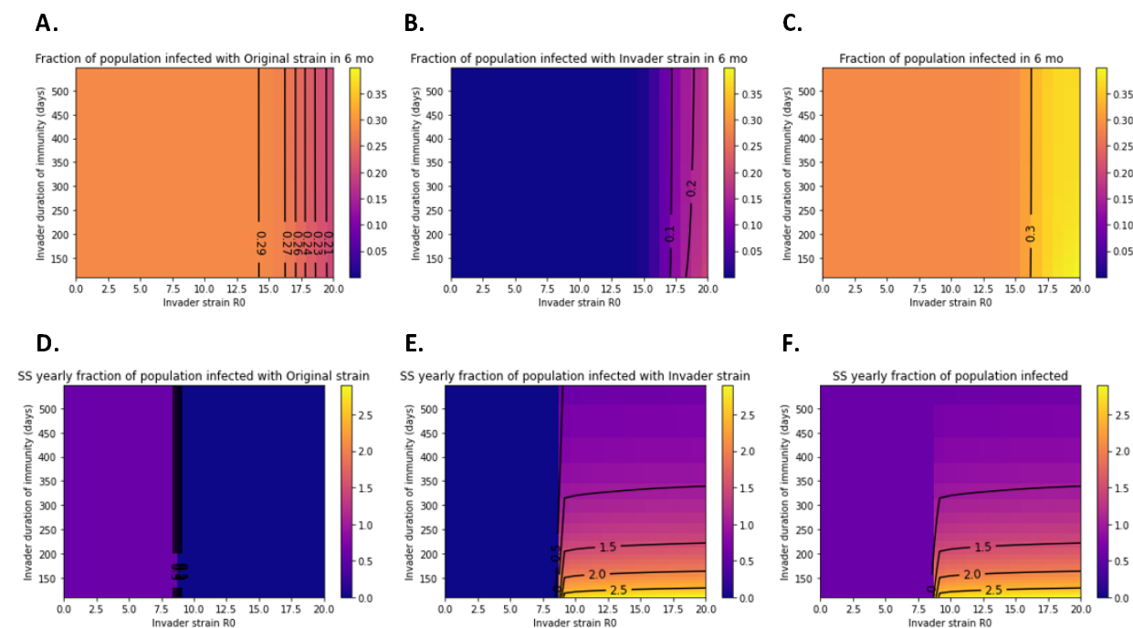
Figure S1. Short-term and long-term transmission trends after introduction of invader strains with varying transmissibility and durability of immunity. The total number of infections is expressed as a fraction of the population size. Fractions greater than 1 indicate reinfection. Total infections over six months due to A) the original strain, B) the invader strain, or C) both summed together. Total infections over one year at steady-state for D) the original strain, E) the invader strain, or F) both summed together. Colormaps are matched across subpanels A-C and D-F.
