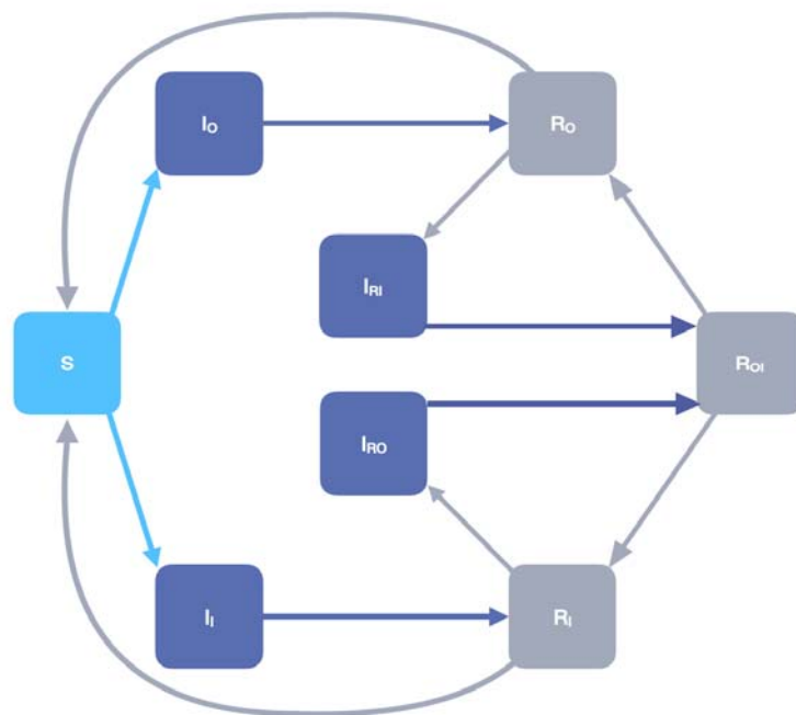
Figure 1. Schematic representing the two-strain SIRS model. Light blue represents fully susceptible individuals, dark blue represents infected individuals, and gray represents recovered individuals.
