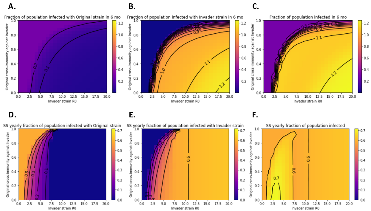
Figure 5. Short-term and long-term transmission trends after introduction of invader strains with varying transmissibility and unilateral cross-immunity properties. The total number of infections is expressed as a fraction of the population size. Fractions greater than 1 indicate reinfection. Total infections over six months due to A) the original strain, B) the invader strain, or C) both summed together. Total infections over one year at steady-state for D) the original strain, E) the invader strain, or F) both summed together. Colormaps are matched across subpanels A-C and D-F.
