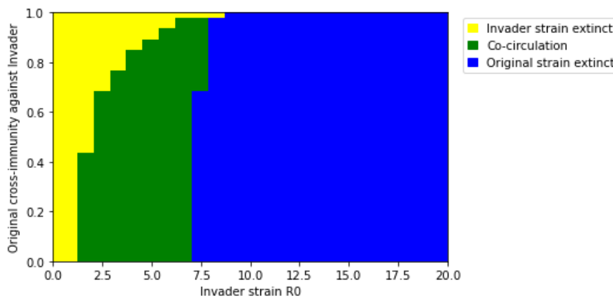
Figure 4. Invasion outcomes for novel variants with varying transmissibility and degrees of asymmetrical immune evasion.
