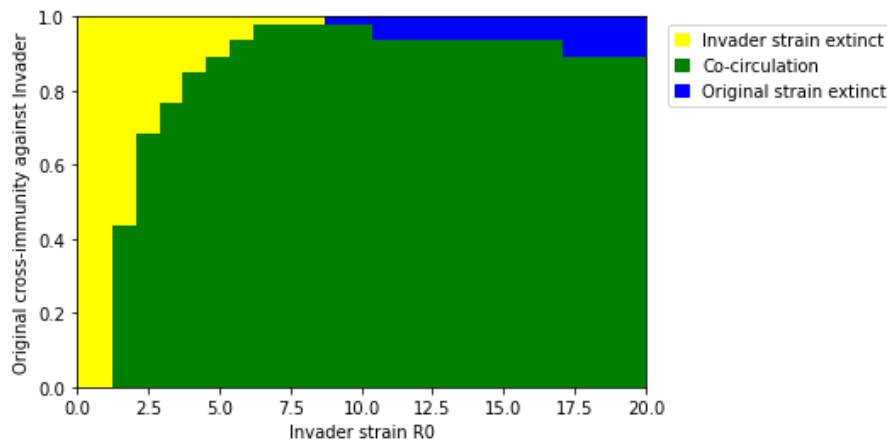
Figure 2. Invasion outcomes for invader strains with varying transmissibility ( R_0 ) and symmetric cross-immunity with the original strain. Outcomes are classified based on whether either strain becomes extinct. Invasion is successful unless the invader strain becomes extinct (yellow).
