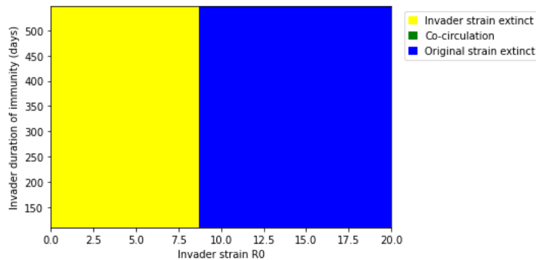
Figure 6. Outcomes for invasion scenarios in which the novel strain induces less durable immunity than the original strain. The duration of immunity against wild-type SARS-CoV-2 infection is estimated to be 550 days [42].
