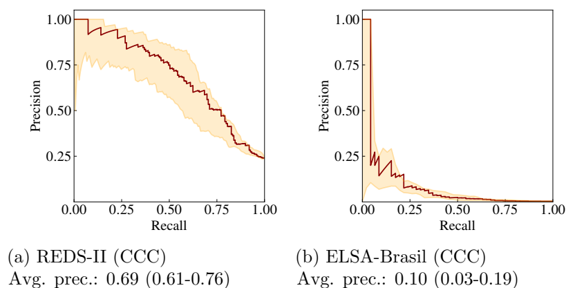
Figure S.2: Precision-recall curves on test data: CCC vs rest. We consider only CCC as positive and ChD as well as normal as negative here.
