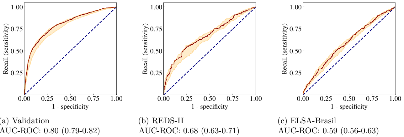
Figure 3: ROC curves on validation and test data: ChD vs normal. Receiver operating characteristics (ROC) computed on the validation data set (SaMi-Trop + CODE) (a) and the test data sets, REDS-II (b) and ELSA-Brasil (c). The shaded regions encapsulate the maximum and minimum values corresponding to 15 different weight initialisations. The outputs of the 15 trained models are averaged to produce the output of the ensemble model, the result of which is shown by the solid lines. The 95% CI is obtained by bootstrapping the ensemble model. The dotted blue lines correspond to completely random assignment of class probabilities.
