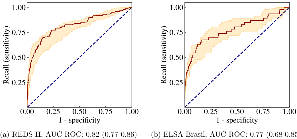
Figure 4: ROC curves on test data: CCC vs all. Receiver operating characteristics computed in REDS-II and ELSA-Brasil for predicting Chagas Cardiomyopathy. The shaded regions encapsulate the maximum and minimum values corresponding to 15 different weight initialisations – the outputs of these models are averaged to produce the output of the ensemble model, the result of which is given by the solid lines. The dotted blue lines correspond to completely random assignment of class probabilities.
