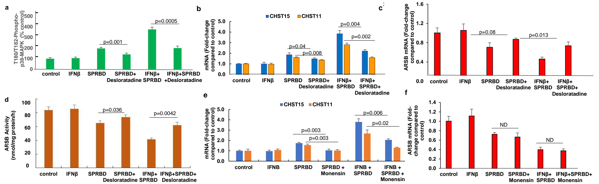
Fig. 4. Effects of desloratadine and monensin on expression of CHST15, CHST11 and ARSB
