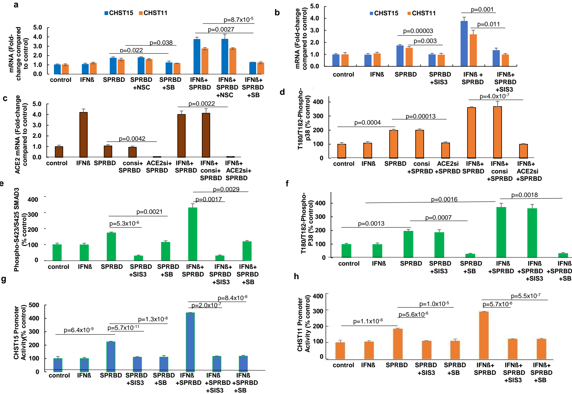
Fig.2. SMAD3 and p38-MAPK inhibitors abrogate the effects of SPRBD.
