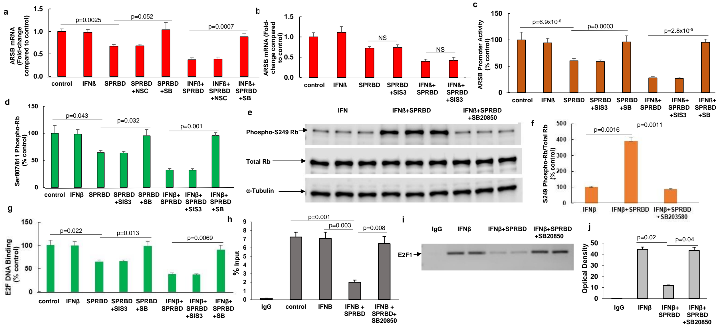
Fig.3. Spike protein receptor binding domain Inhibits ARSB activity and expression by activation of phospho-p38 MAPK and phospho-(S249/T252)-RB-E2F1 interaction.
