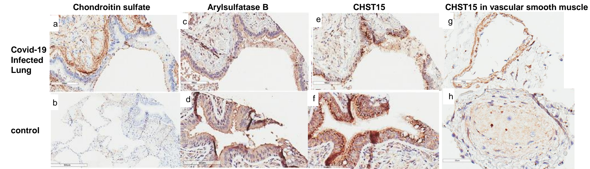
Fig. 1. Chondroitin sulfate, Arylsulfatase B, and CHST15 in Covid-19 and normal control lung tissue and in human small airway epithelial cells.
