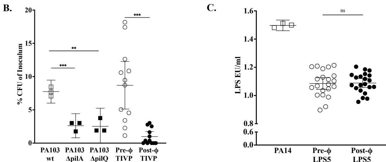
Figure 2. Effect of Phage Therapy on Pseudomonas Antibiotic Resistance and Virulence. (A). Effect of Phage Therapy on Pseudomonas Antibiotic Resistance. Phage therapy with OMKO1, which targets Pseudomonas efflux pumps, results in increased antibiotic sensitivity. In two Subjects (#1 and #3) who received OMKO1 phage therapy, Pseudomonas aeruginosa antibiotic sensitivity testing completed from clinical laboratories is shown comparing pre- and post-phage therapy. Subject #1 two isolates reported pre- and post-phage therapy. Subject #3 one isolate pre-phage therapy compared to three isolates post-phage therapy. S = sensitive, I = intermediate, R = resistant, and X = not reported. (B). Effect of Phage Therapy on Pseudomonas Virulence. (B) Pseudomonas aeruginosa attachment to CF airway epithelial (CFBEo-) cells was measured. Bacteria from different Pseudomonas laboratory strains wildtype (WT) PA103, PA103 TIVP mutants PA103 \Delta pilA and PA103 \Delta pilQ, and four (4) PsA isolates pre-TIVP-H6 phage (Pre- \phi ) and three (3) PsA isolates post-TIVP-H6 phage (Post- \phi ) TIVP from Subject 2 (the only individual who received TIVP-H6 single phage therapy). Each isolate was added to CFBEo- cells at air-liquid interface and attachment was measured in triplicates (CFU percentage of the original inoculum). PA103 WT vs. PA103 \Delta pilA; N = 1-2, in triplicate (** p < 0.001 ; Welch's t test); PA103 WT vs. PA103 \Delta pilQ; N=1-2, in triplicate (** p < 0.01 ; Welch's t test). Pre- \phi vs. post- \phi TIVP phage therapy isolates; N = 3-4, in triplicate (** p < 0.001 ; Welch's t test). (C) Endotoxin was measured in Pseudomonas aeruginosa supernatants after LPS phage therapy. LPS EU/ml was measured (corrected for CFU/ml) in a Pseudomonas laboratory strain (PA14) and pre- and post-LPS phage cell-free PsA supernatants from Subjects 4 and 5 (individuals who received LPS-5 single phage therapy), N = 7, in triplicate (comparison was non-significant; Welch's t test).
