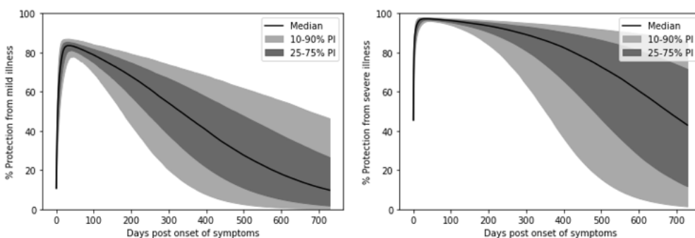
Figure 2: Post-infection protection from mild and severe COVID-19 outcomes. Protection is calculated against strain inducing immunity – that is, immune evasion is not accounted for. Protection over time will be further eroded by immune evasion.
