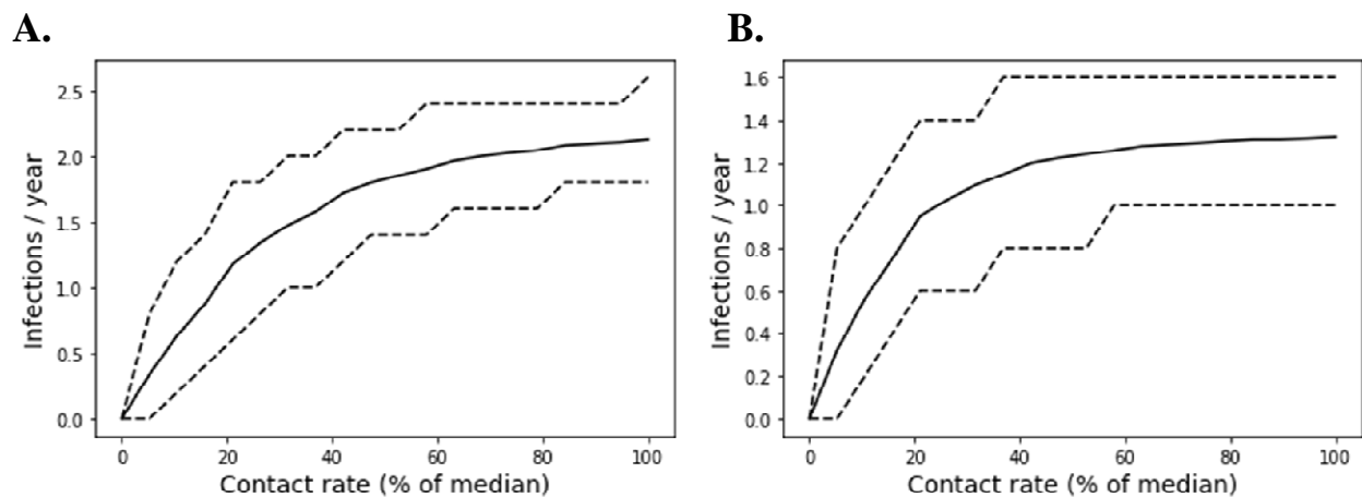
Figure 5: Frequency of infection (infections per year) is nonlinearly associated with individual contact rates. Infection frequencies among A. unvaccinated individuals and B. vaccinated individuals. Only individuals restricting their contact rates to less than 25% of the median achieve reductions in infection frequency. Solid lines represent the mean outcome while dashed lines delineate the 90% population interval.
