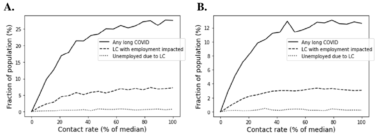
Figure 6. An individual’s long COVID risk decreases nonlinearly with reductions in contact rate. Fraction of A. Unvaccinated individuals and B. vaccinated individuals experiencing long COVID of varying severity at any given time as a function of individual contact rate.
