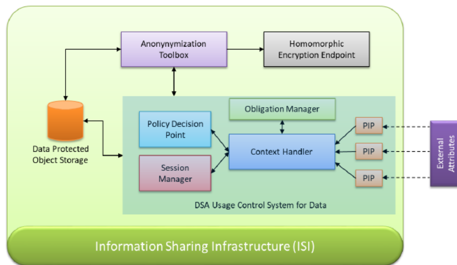
Figure 5 Information Sharing Infrastructure (ISI)
