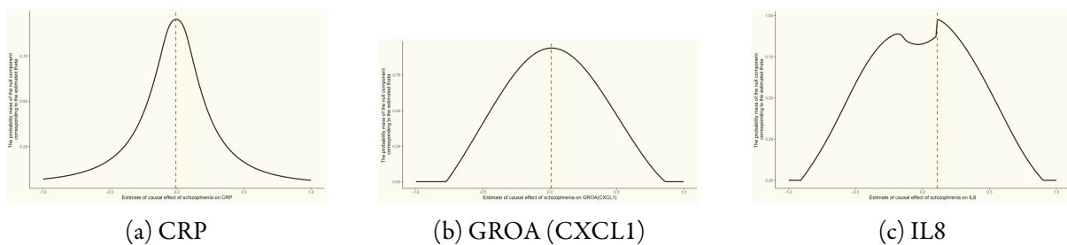
Fig. 6: Grid search of possible causal effects (theta) of schizophrenia on CRP, GROA (CXCL1) and IL8; the maroon vertical line pointing to the theta which leads to maximum \pi_0
