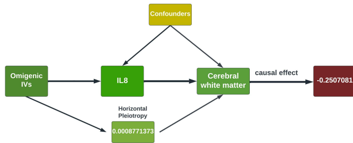
Fig. 5: Estimates of the nominally significant casual effect of IL8 on the linear change rate of cerebral white matter
