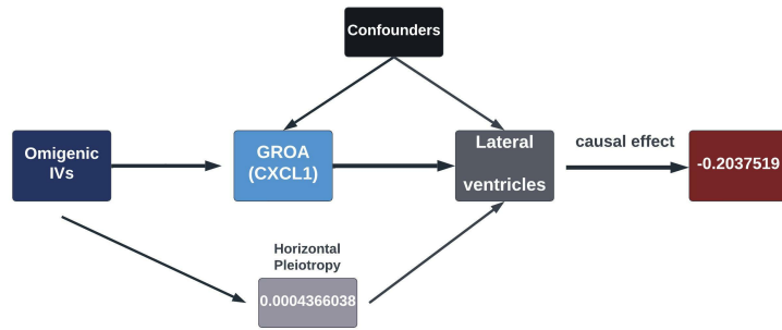
Fig. 4: Estimates of the nominally significant casual effect of GROA (CXCL1) on the linear change rate of lateral ventricles
