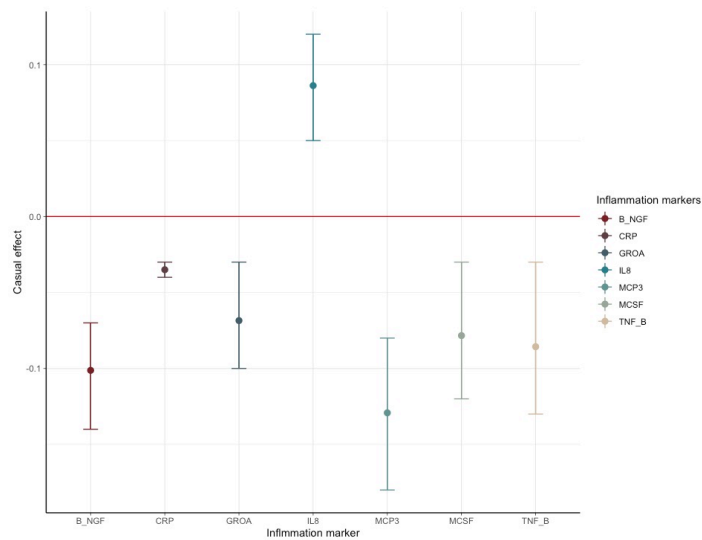
Fig. 2: Causal estimates of seven inflammation markers responding significantly to schizophrenia
