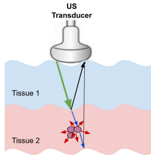
Figure 1: Ultrasound interaction with tissues. The green, black, red, blue arrows represent the incident wave, the specular reflection, the non-specular reflection, and the refracted wave, respectively.
