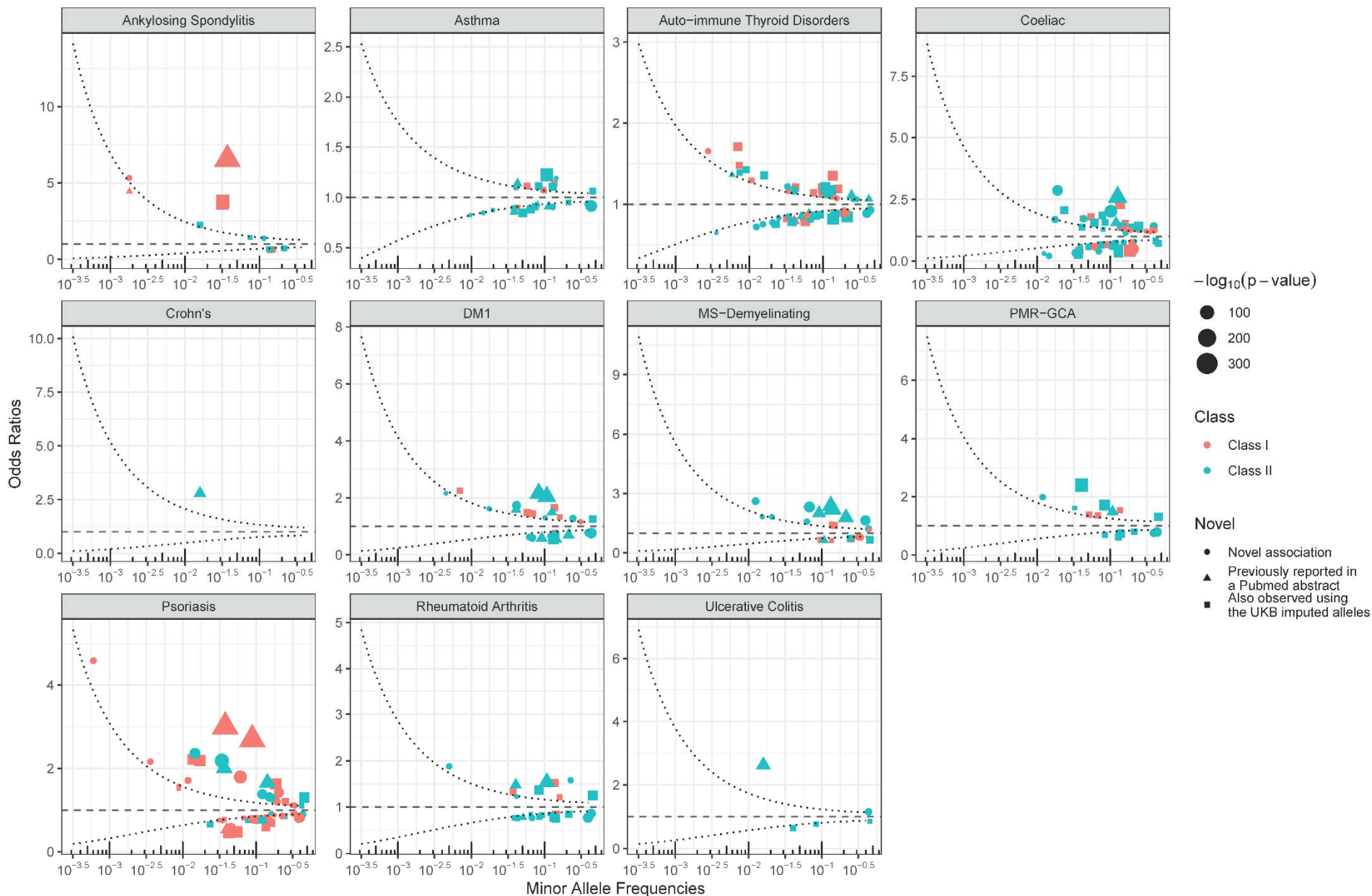
Fig. 3: HLA association studies at 2-field resolution. Odds ratios are shown. The curved dashed lines represent a power of 80% to detect an association at a p-value of (5 \times 10^{-8})/11 or less. Circles show likely novel allele associations. Pertinent positive controls include HLA-B*27:05 for ankylosing spondylitis (OR: 6.55, 95% CI: 5.97 – 7.18, p = 1.97 \times 10^{-305} , EAF: 3.9%). Also note the rare and novel allele associations HLA-B*57:31 for psoriasis (OR = 4.61, 95% CI: 3.22 – 6.59, p = 7.1 \times 10^{-17} , EAF = 0.06%), and HLA-C*02:178 for ankylosing spondylitis (OR = 5.33, 95% CI: 3.37 – 8.41, p = 7.75 \times 10^{-13} , EAF = 0.2%). For 3-field resolution results, refer to supplementary figures SF5 .
