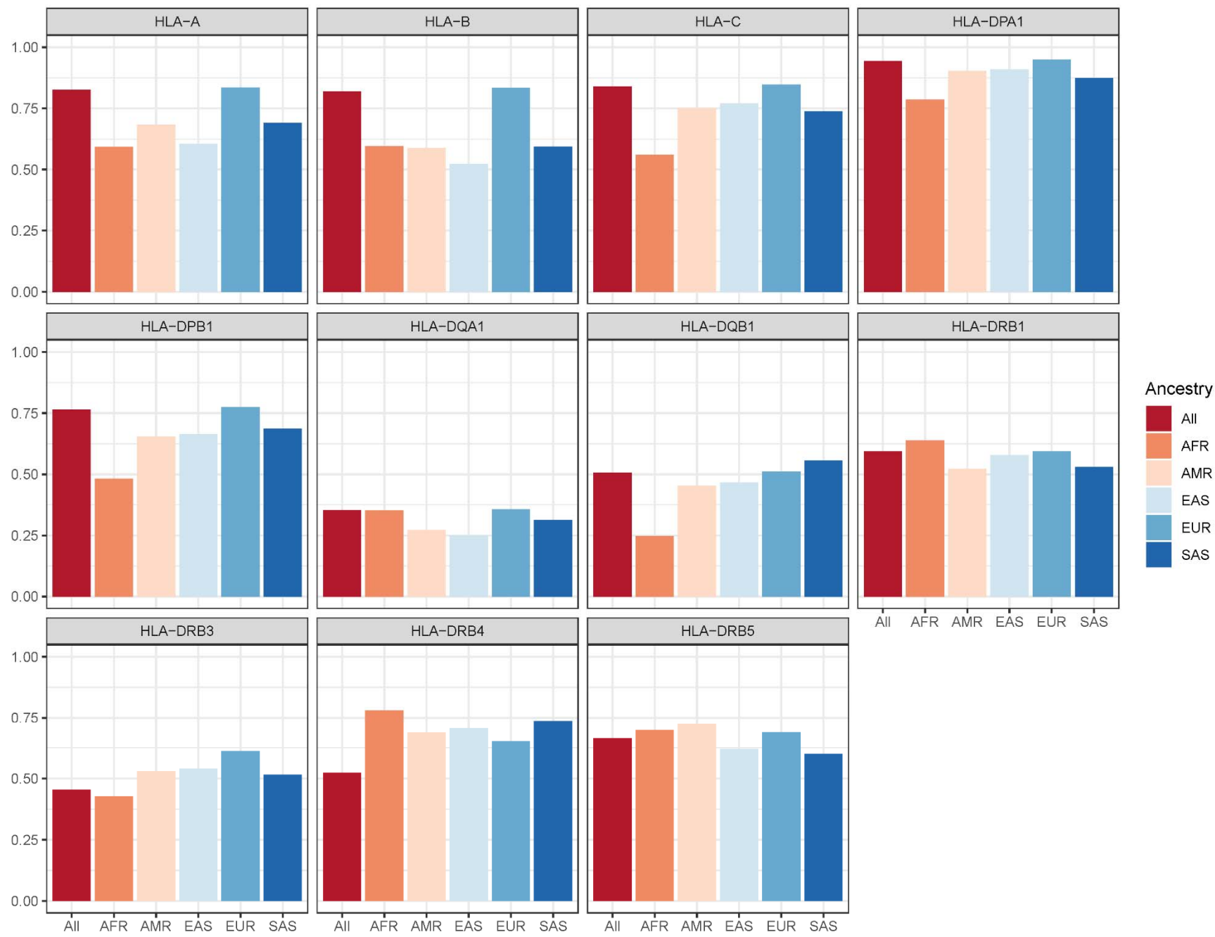
Fig. 2: Concordance (%) between sequenced and imputed HLA alleles stratified by HLA genes and genetic ancestry.
