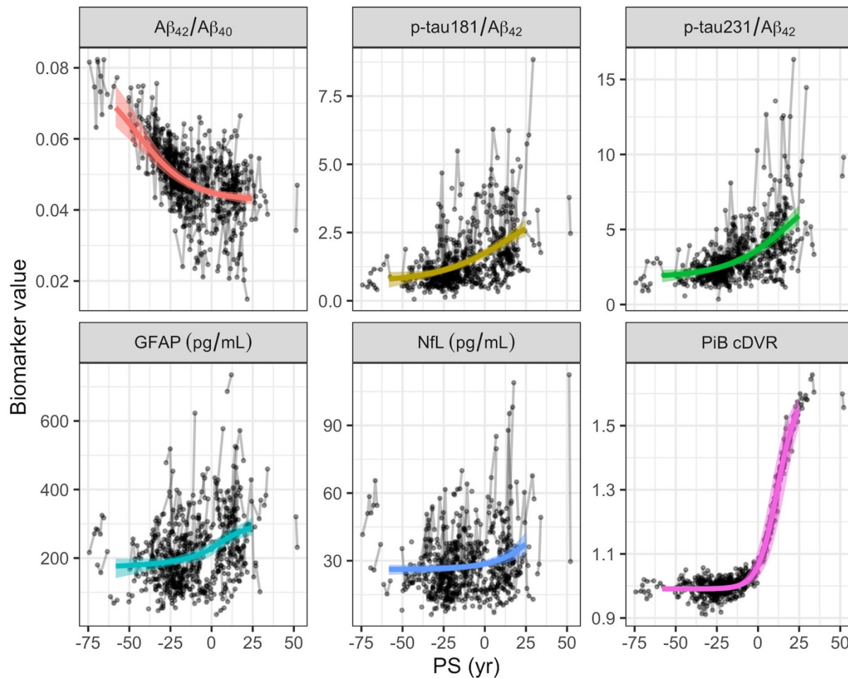
Figure 3: Biomarker trajectories estimated after alignment of individual-level longitudinal data using the progression score (PS) model. Bands indicate the 95% confidence intervals for the trajectory estimates. PS scale was calibrated after model fitting such that at PS = 0 , the estimated trajectory for PiB cDVR attains the value 1.06, which is the PiB positivity threshold. Since PS is time-shifted age, it is in the units of years. A\beta , amyloid- \beta ;
