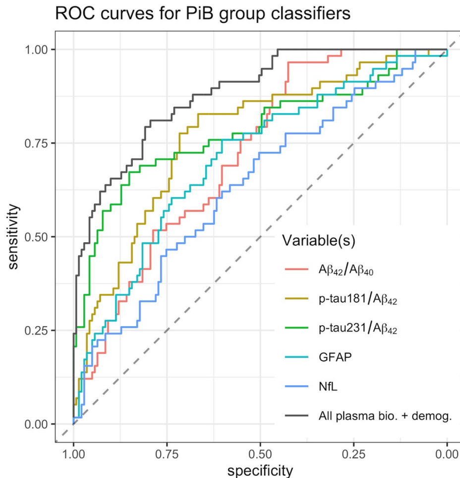
Figure 1: Receiver operating characteristic curves for univariate classifiers and the best multivariable classifier (including all plasma measures, age, sex, race, and APOE \epsilon 4 status as features) for predicting PiB group. A\beta , amyloid- \beta ; APOE, apolipoprotein E; bio., biomarkers; demog., demographics; GFAP, glial fibrillary acidic protein; NfL, neurofilament light chain; PiB, Pittsburgh compound B; p-tau, phosphorylated tau; ROC, receiver operating characteristic.
