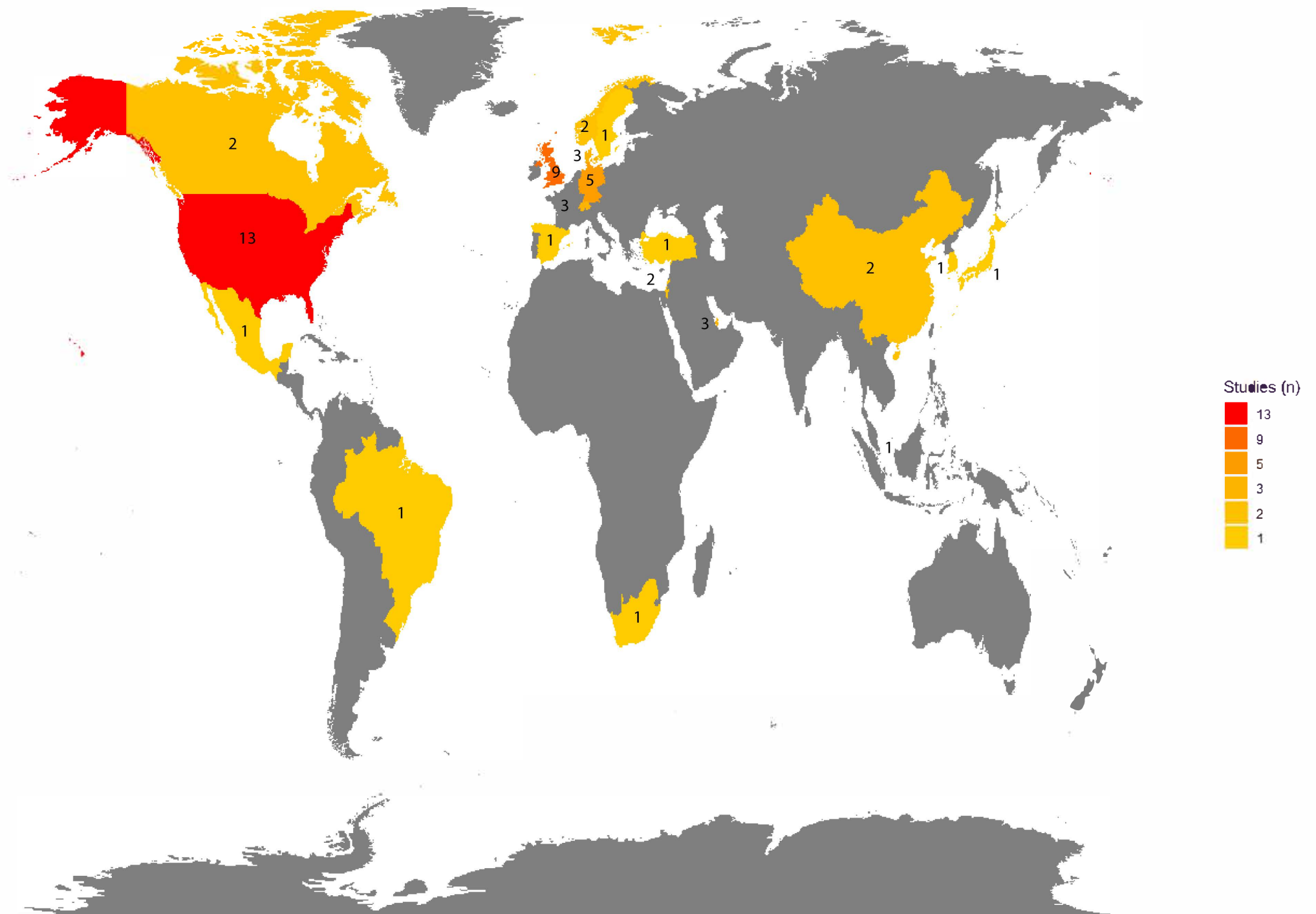
Figure 2. Map of the number of studies conducted in each country
