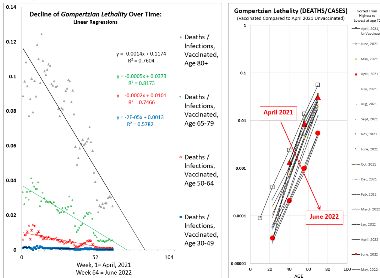
FIGURE 4 Decline in Gompertzian Lethality April 2021 to June 2022, USA, by age. 14 (Left) Linearly, date on X-axis; (Right) Logarithmically, age on X-axis
