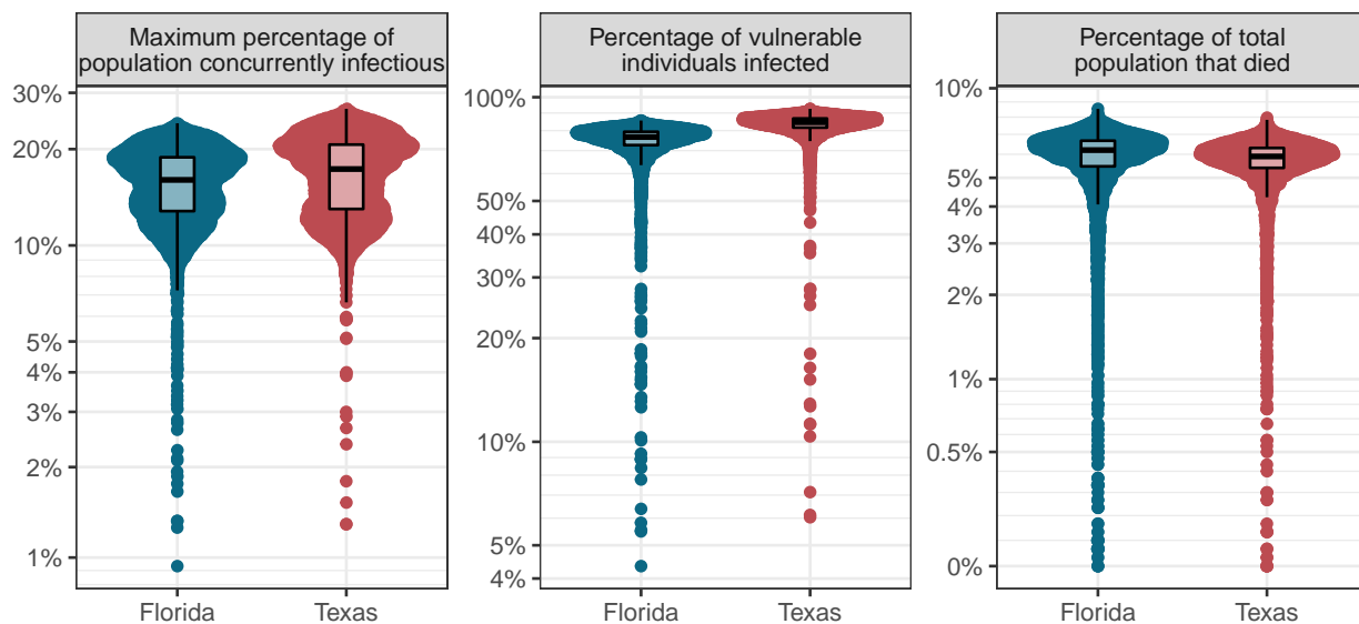
Figure S3: As fig. 2 in the main text, but with no background transmission. Comparing the difference in peak proportion infectious, overall prevalence among vulnerable individuals, and overall mortality between simulations of epidemics in two possible population structures, as characterized by age- and household-size distributions. Only simulations with no difference in behaviour based on vulnerability and only outcomes from epidemics resulting in greater than 5% of the total population being infected are shown.
