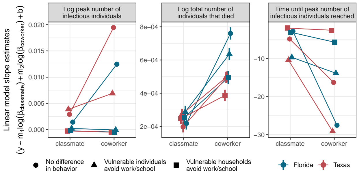
Figure S7: As figs. 3 and S4, but with background transmission set to \beta_{background} = 0.1/N .
