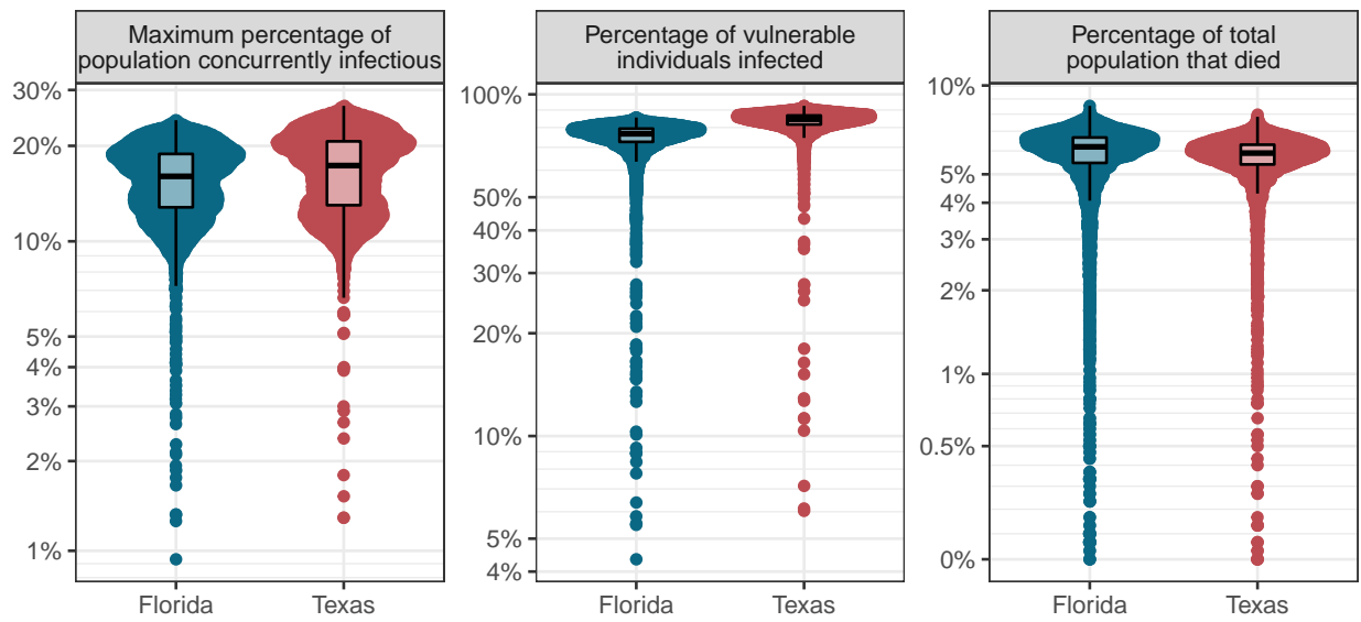
Figure S6: As figs. 2 and S3, but with background transmission set to \beta_{background} = 0.1/N .
