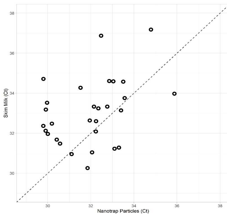
438 Figure 5. Comparison of automated Nanotrap particle method for processing 10 mL Moore swab 439 wastewater vs. skim milk method for processing of 250 mL Moore swab wastewater for 440 detection of SARS-CoV-2 RNA.
