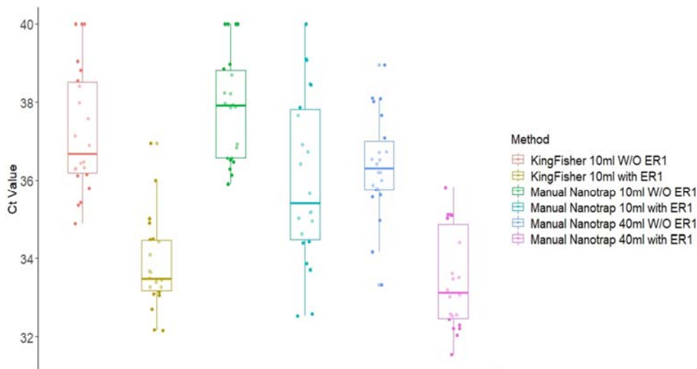
420 Figure 2. Comparison of SARS-CoV-2 RNA detection in 10 mL grab wastewater samples from 421 influent lines processed using the automated Nanotrap particle method and the manual Nanotrap 422 particle method (10 mL and 40 mL) with and without ER1.
