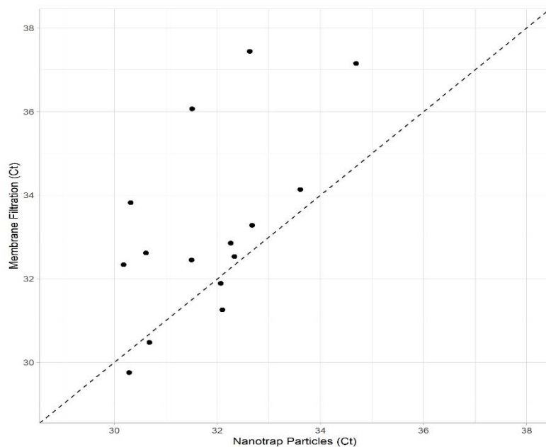
434 Figure 4. Comparison of automated Nanotrap particle method and ER1 for processing 10 mL 435 grab wastewater with vs. membrane filtration method for processing of 150 mL wastewater in 436 detection of SARS-CoV-2 RNA.
