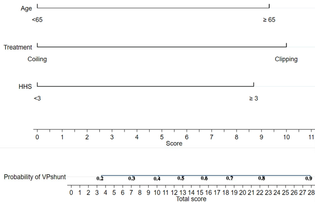
Figure 1. Nomogram plot for predicting SDHC aSAH patients. For an individual patient, each variable corresponds to a point in the fourth row (Score: 0-11). The total points can be summed up by points of 3 variables and indicated in the sixth row (the bottom row: 0-28). The probability of SDHC for individual patient can be evaluated by drawing a vertical line from a total point to the fifth row (Probability of VP shunt: 0.2-0.9).
