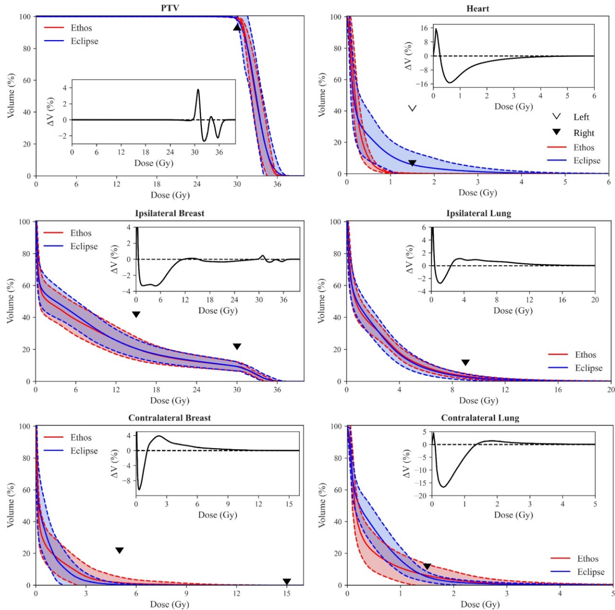
Figure 3 | Population DVH comparison of Eclipse manual and Ethos automatic plans. Shaded areas show the mean \pm standard deviation of all validation cohort data, and the inferior/superior point of triangles illustrate RAD 1802 planning objectives. Insets show the difference between mean population DVHs (i.e., Ethos mean volume minus Eclipse mean volume). Inset axes were sized for optimal visualization.
