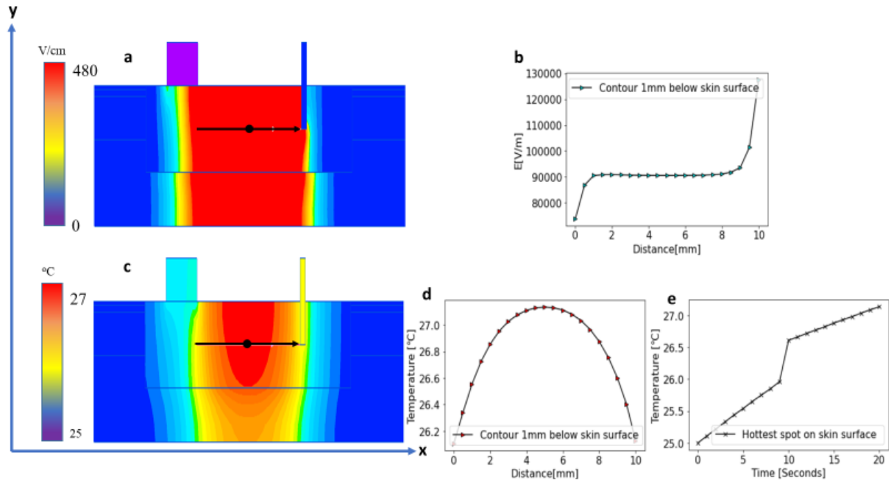
Figure 3 (a) The electric field distribution in a lesion while applying 1000V, with a color map of the electric field strength. Red color represents the electroperated tissue area ( E > 480\text{V cm}^{-1} ), which is mainly located between ground and needle electrodes. (b) An electric field strength profile between ground electrode to needle electrode, 1mm below lesion surface (c) Analysis of temperature distribution after two sequential pulses, high and rapid followed by slow and longer pulses. Transient heat transfer problem created through coupling of DC conduction problem when V=1000\text{SV} were applied, V_{\text{rms}} = 12.65\text{V} , pulsing for 10 seconds, with steady state heat transfer problem with confined Dirichlet boundary conditions. The described transient heat problem was coupled after 10 seconds pulsing, with another DC conduction problem when V=50\text{V} were applied, V_{\text{rms}} = 10\text{V} , pulsing for 10 seconds to create a transient heat transfer problem performed in a and d figures. (d) The temperature profile from the ground electrode until the needle electrode. e Temperature increase in time at the point located 1mm beneath the electrode.
