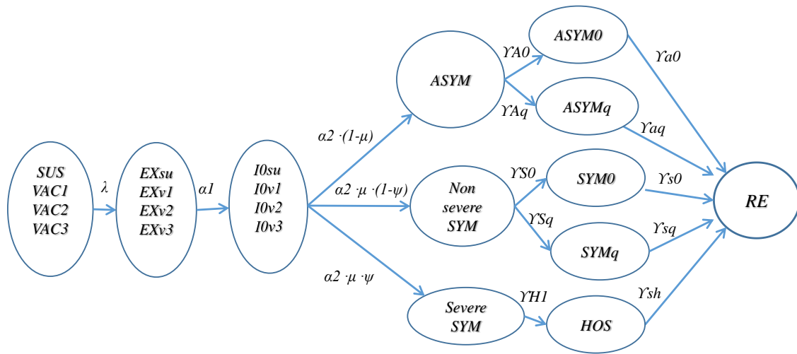
Fig s1: Modelling COVID-19 (omicron) epidemics in China – main compartments and transitions across status
