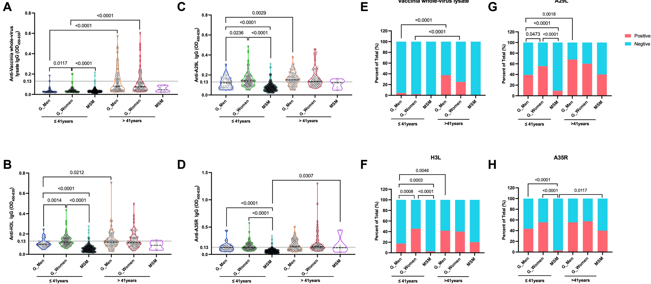
Figure 1 Comparisons of binding IgG antibodies against MPXV H3L, A29L, A35R proteins and vaccinia whole-virus lysate
