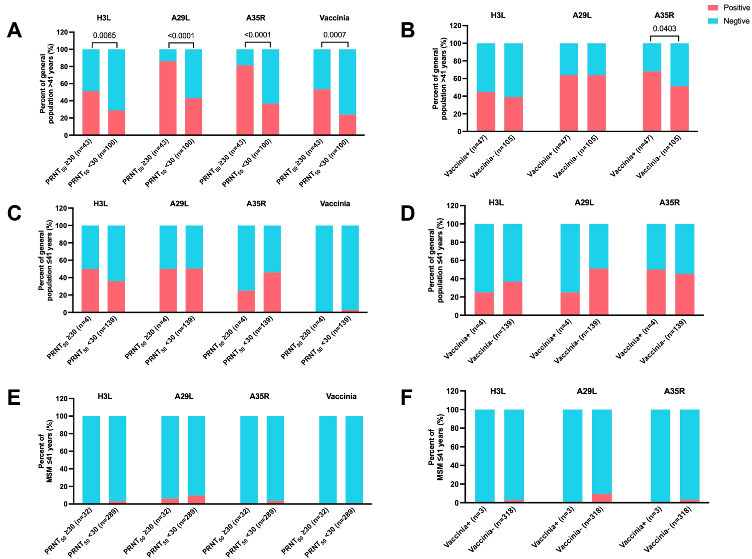
Figure 3 The binding antibody responses against MPXV H3L, A29L and A35R were not associated with the binding and neutralizing antibody responses against vaccinia Tiantan virus among participants ages \leq 41 in both cohorts
