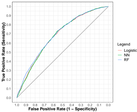
Fig. B1: ROC curves for LOS prediction in validation set.
