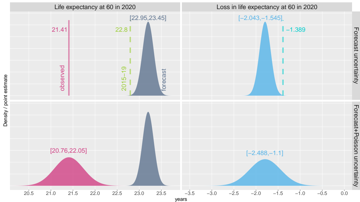
Figure 1: Illustrative figure of sources of uncertainty around excess mortality measure. Life expectancy at 60 (left panels) and associated losses (right panels) for Territoire de Belfort , males, 2020. Upper panels: forecast uncertainty is accounted. Lower panel: both forecast and Poisson uncertainty are reported. Texts refer to either point estimates or 95% confidence intervals. Dashed lines depict naive estimation of excess mortality.
