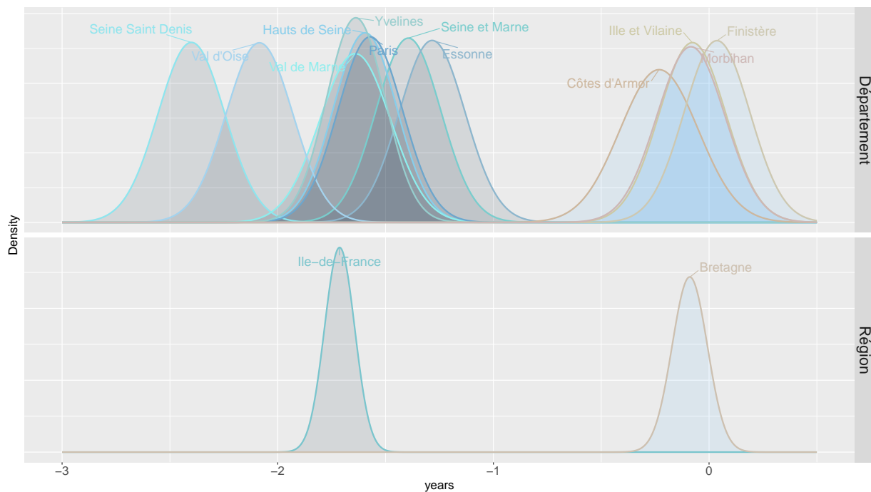
Figure 5: Illustrative figure on the effects of spatial aggregation in excess mortality estimation. Densities of losses/gains in life expectancy at 60 for two NUTS 2 populations ( Ile-de-France and Bretagne , lower panel) and their associated NUTS 3 populations (upper panel).
