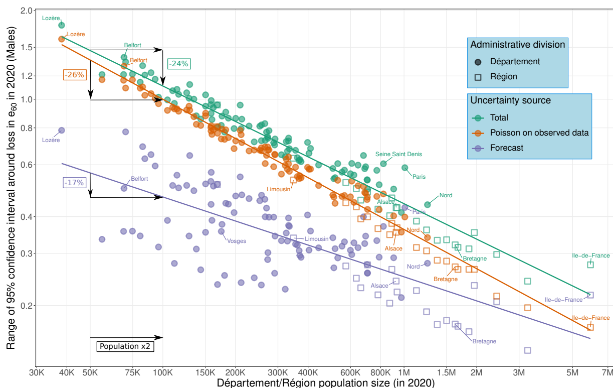
Figure 4: Log-log plot of the amount of uncertainty against population size by source of uncertainty: Total, associated to the Forecast process and due to Poisson randomness in observed data. Uncertainty is measured by the width of the 95% confidence intervals around estimated loss in male e_{60} . Values for both départements (NUTS 3) and régions (NUTS 2) are depicted. Linear fits are provided for illustrative purposes and for obtaining an approximated value of the elasticity associated to each source of uncertainty.
