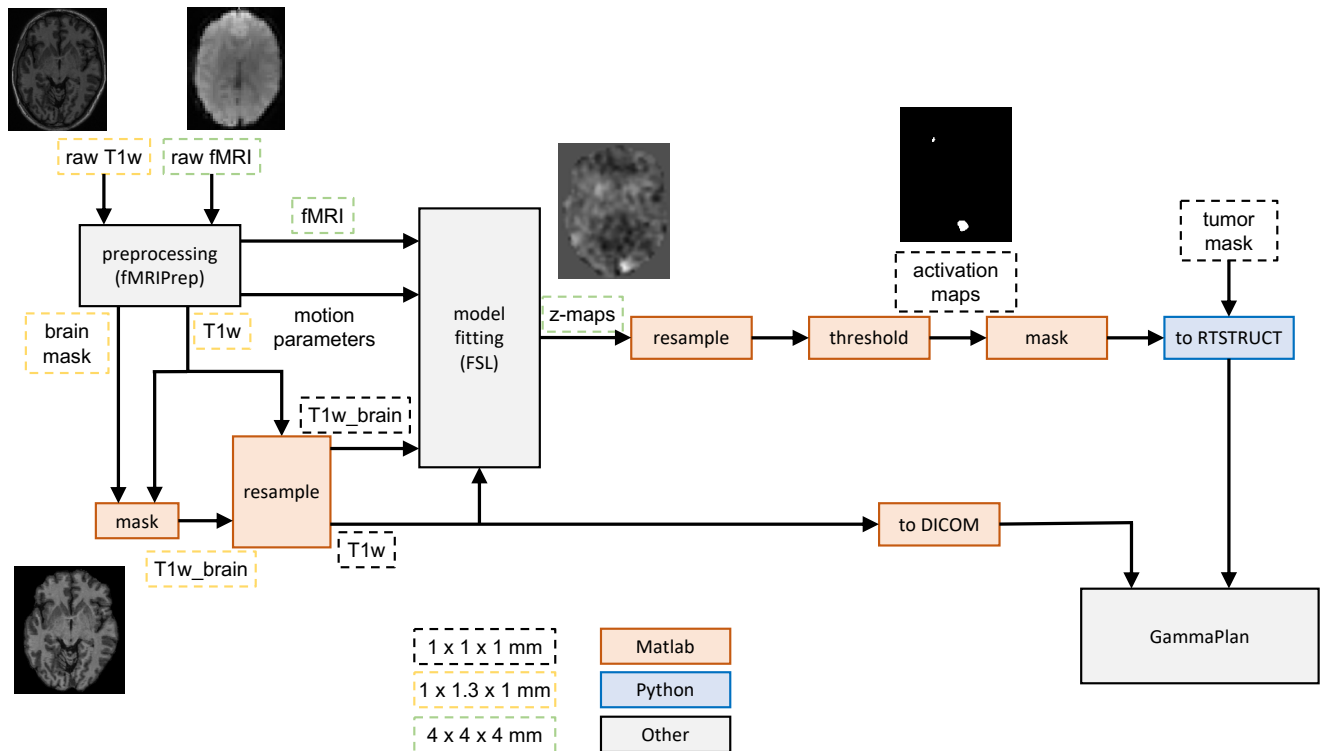
Figure 2: Diagram of the preprocessing and statistical analysis pipeline for fMRI data. The preprocessing (e.g., registration between T1w and fMRI volumes, head motion correction) is done with the fMRIPrep software, with some additional resampling of the volumes. The statistical analysis of the fMRI data is done with the FSL software. A custom Python script is finally used to convert the brain activity maps to DICOM RTSTRUCT, for loading them into GammaPlan.
