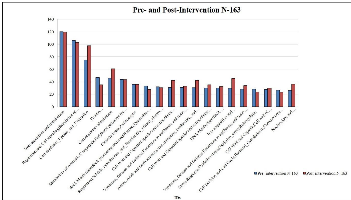
Figure 5: SEED-based functional analysis of metabolic and functional pathways
