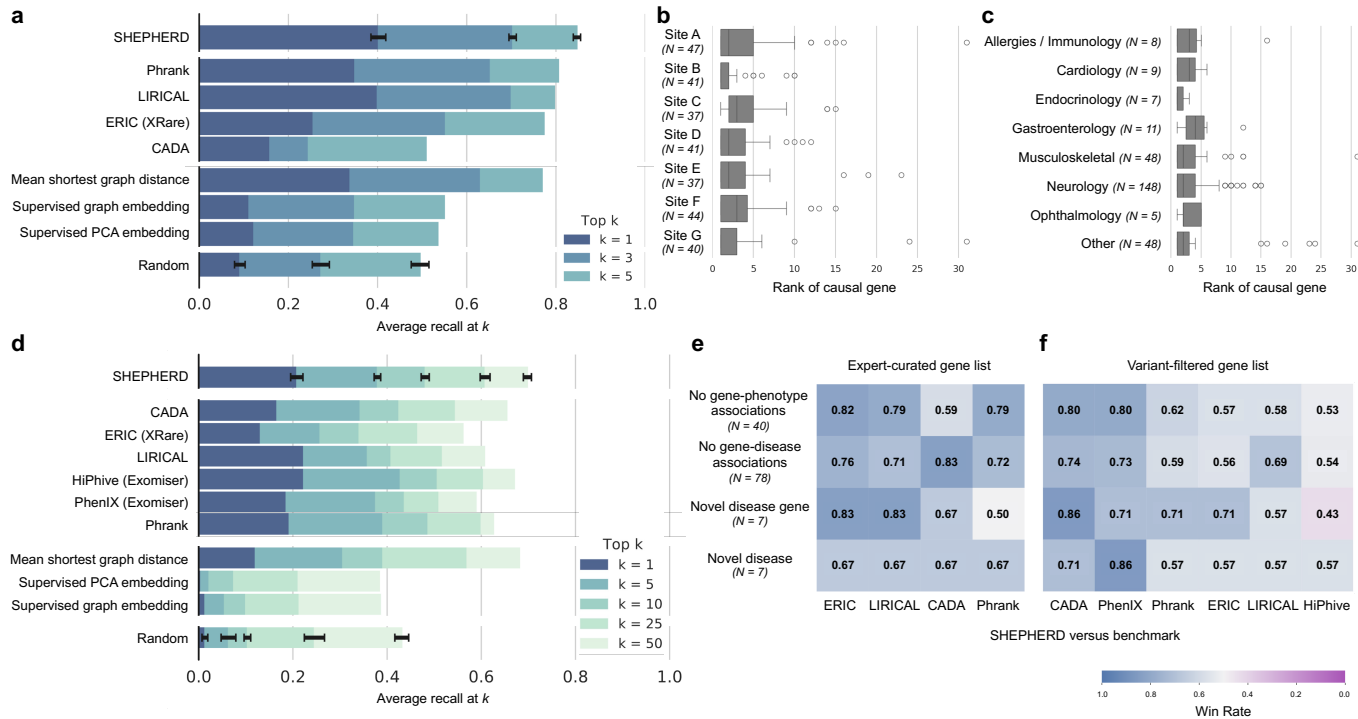
Figure 3: SHEPHERD performs generalizable causal gene discovery. (a) Performance of SHEPHERD, four domain-specific approaches, three traditional machine learning / network science baselines, and a random baseline. The performance metric is average recall at k for k = 1, 3, and 5 . Error bars denote standard deviation over models trained with 5 random seeds. (b-c) Performance of SHEPHERD in ranking causal genes stratified by (b) clinical sites and (c) primary presenting symptoms. Each boxplot shows the median and interquartile range of the rank of the causal gene. Whiskers extend to \pm 1.5 \times IQR. (d) Performance of SHEPHERD, six domain-specific approaches, three traditional machine learning / network science baselines, and a random baseline. The performance metric is average recall at k for k = 1, 5, 10, 25, and 50 . Error bars denote standard deviation over models trained with 5 random seeds. (e-f) Performance of SHEPHERD against domain-specific algorithms in four extremely hard-to-diagnose scenarios on (e) EXPERT-CURATED and (f) VARIANT-FILTERED gene lists. Shown is the win rate, the proportion of patients where SHEPHERD performs the same as or better than the benchmark algorithms.
