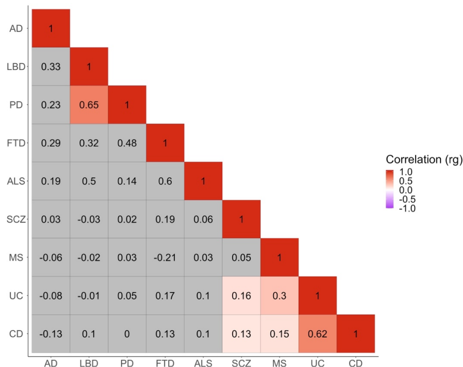
Figure 1. Genome-wide genetic correlations ( r_g ) across GWAS traits. Significant positive correlations (Bonferroni corrected p -value < 0.0014 ) are highlighted in shades of red. AD = Alzheimer’s disease; LBD = Lewy body dementia; PD = Parkinson’s disease; FTD = Frontotemporal dementia; ALS = Amyotrophic lateral sclerosis; SCZ = Schizophrenia; MS = Multiple sclerosis; UC = Ulcerative colitis; CD = Crohn’s disease.
