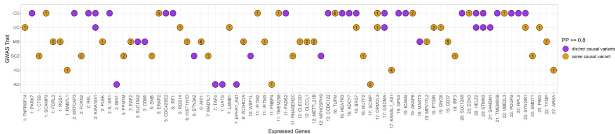
Figure 5. Colocalization results between diseases and expressed genes in at least one immune cell type. Pairs of traits that share a causal variant through colocalization analysis are highlighted in orange (Posterior Probability, PP H4 \geq 0.8 ), whereas pairs of traits that have distinct causal variants are highlighted in purple ( PP H3 \geq 0.8 ). The number inside the colocalized signals indicates the number of cell types for which a colocalization was observed. The cell type(s) for each disease-gene pair displayed here are listed in Supplementary Table 4.
