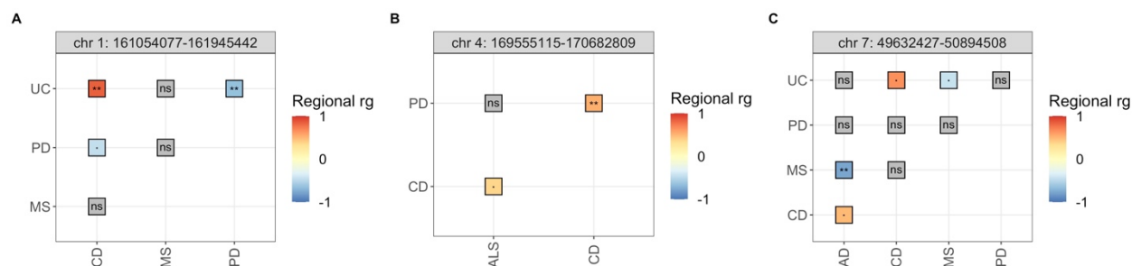
Figure 2. Significant regional genetic correlations ( r_g ) between neurodegenerative and immune-mediated diseases across three distinct loci in chromosomes 1 (A), 4 (B) and 7 (C). ** = significant correlations ( p -value < 2.629e-05 ); · = nominally significant correlations; ns = non-significant correlations ( p -value \geq 0.05 ). Absence of correlations means that the bivariate test was not performed (See Methods for details). CD = Crohn’s disease; MS = Multiple sclerosis; UC = Ulcerative colitis; PD = Parkinson’s disease.
