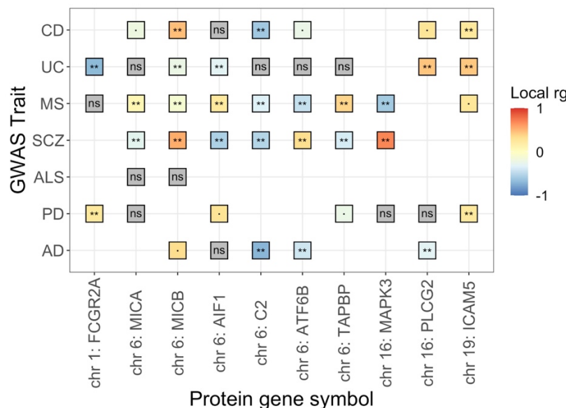
Figure 6. Regional correlations between protein levels and diseases shared between at least one test disease (i.e., AD, PD, ALS, LBD, FTD, SCZ) and at least one control disease (i.e., MS, UC, CD). ** = significant correlations ( FDR < 0.01 ); · = nominally significant correlations; ns = non-significant correlations ( p\text{-value} \geq 0.05 ).
