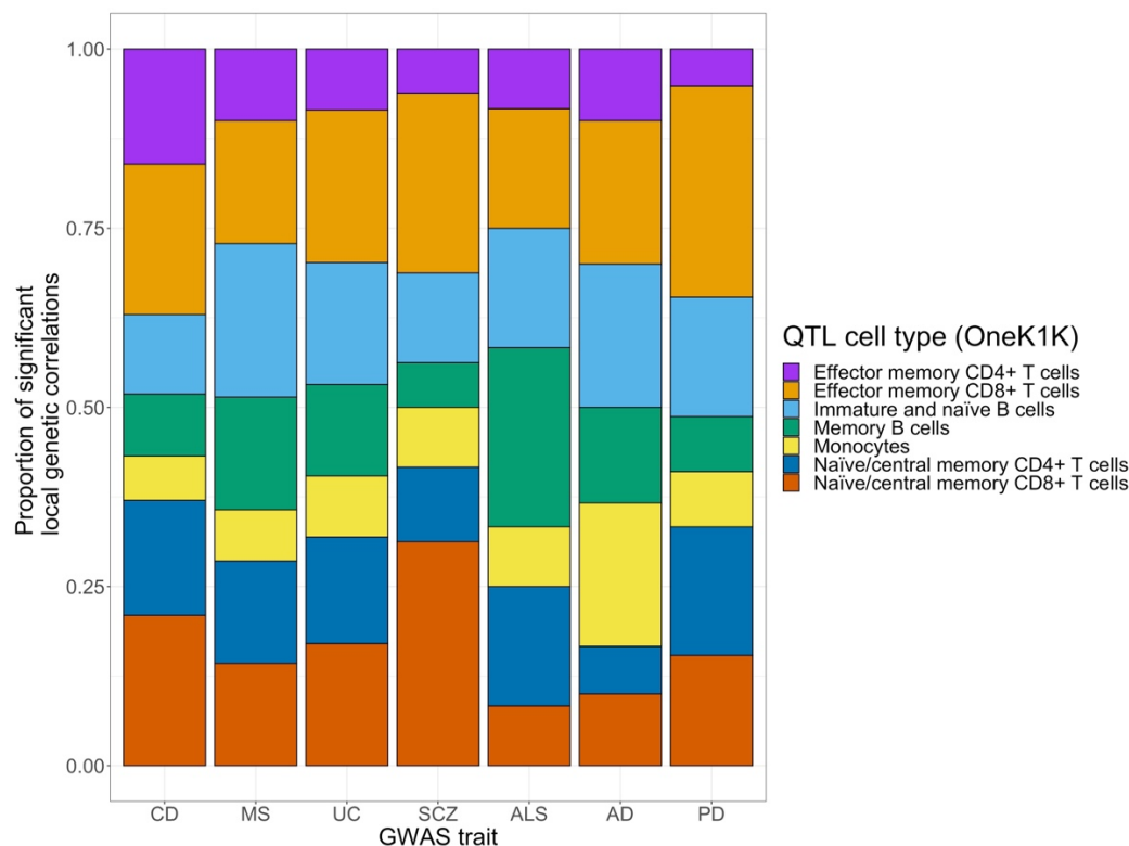
Figure 3. Proportion of significant regional genetic correlations between diseases and gene expression, across seven immune cell types. As there were no significant correlations for neither frontotemporal dementia nor Lewy body dementia, those traits are not displayed. CD = Crohn’s disease; MS = Multiple sclerosis; UC = Ulcerative colitis; SCZ = Schizophrenia; ALS = Amyotrophic lateral sclerosis; AD = Alzheimer’s disease; PD = Parkinson’s disease.
