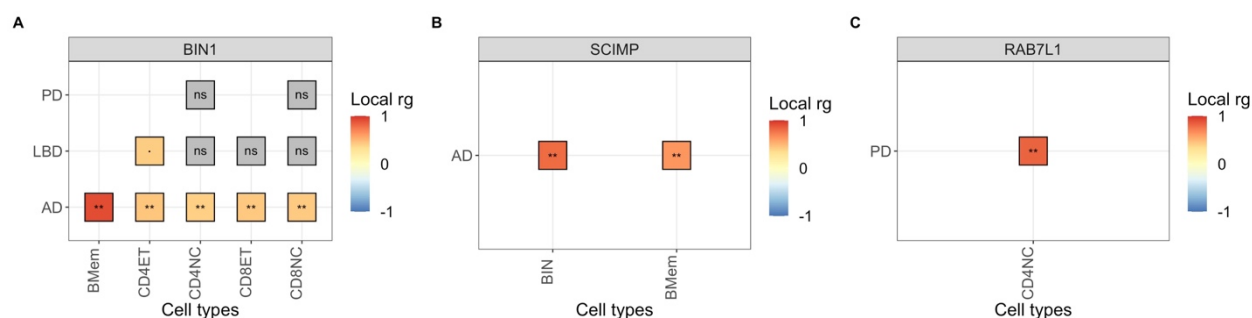
Figure 4. Examples of significant regional correlations between gene expression levels and diseases across three genes. (A) BIN1 (chromosome 2) was significantly correlated with AD across various adaptive immune cell types. (B) SCIMP (chromosome 17) was significantly correlated with AD across B cells. (C) RAB7L1 (chromosome 1) was significantly correlated with PD in naive CD4+ T cells. ** = significant correlations (FDR < 0.01); · = nominally significant correlations; ns = non-significant correlations (p-value \geq 0.05). AD = Alzheimer’s disease; LBD= Lewy body dementia; PD = Parkinson’s disease; BMem = Memory B cells; CD4ET = CD4+ effector memory T cells; CD4NC = CD4+ naive T cells; CD8ET = CD8+ effector memory T cells; CD8NC = CD8+ naïve T cells.
