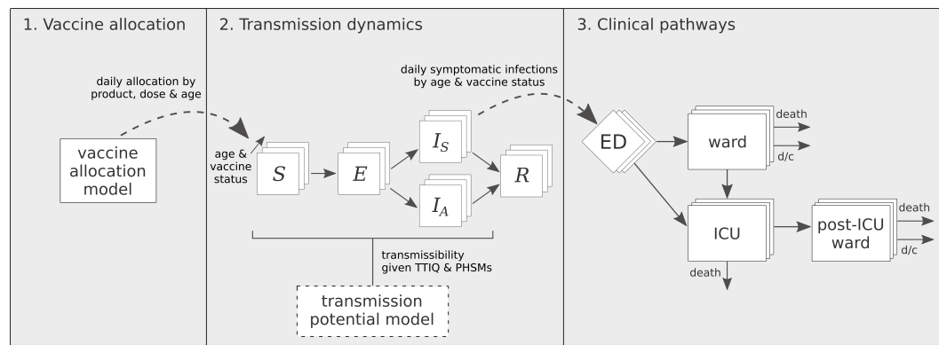
Figure 1. Schematic of three interlinked model components. 1. A model of vaccine allocation and roll-out to the Australian population (aged 16 and over). 2. An age-structured individual-based model of SARS-CoV-2 transmission dynamics to model infection numbers by age and vaccine-status. Note that transmissibility of SARS-CoV-2 under different PHSM bundles and TTIQ capabilities is informed by outputs from a model of SARS-CoV-2 transmission potential described in [10]. 3. A clinical-pathways stochastic model to map infection numbers to hospital admissions, ward and ICU occupancy, and deaths stratified by age and vaccine-status. S = susceptible; E = exposed; I_S = infectious and develops symptoms; I_A = infectious and does not develop symptoms; R = recovered; ED = emergency department, ICU = intensive care unit; d/c = discharge.
