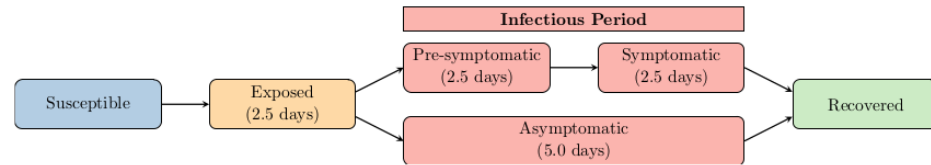
Figure S2. Transmission model: a simple schematic describing the mutually-exclusive states that an individual may reside in, and the transition between those states.
