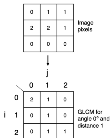
Fig. 4. GLCM transformation on 3x3 arrangement of pixels with values 0-2. Performed on 0° angle and pixel distance 1.
