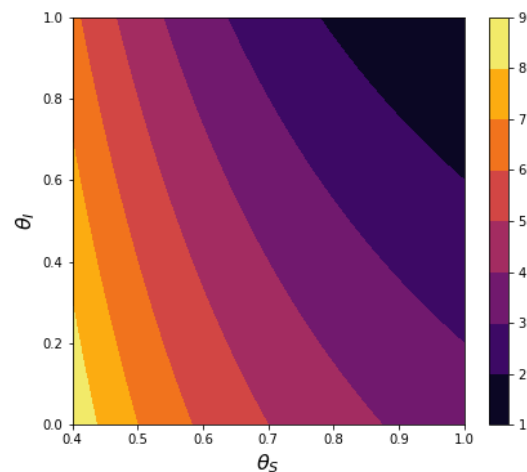
Figure S5: \hat{\theta}_E (the value of the relative contribution to escape from the vaccinated above which intermediate coverages maximise the escape pressure) in the endemic scenario, as given by (19). We only plot values of the susceptibility VE \theta_S above 0.4, because \hat{\theta}_E quickly grows without bounds as \theta_S \rightarrow 0 (the vaccines become better at preventing infection). In other words, \hat{\theta}_E is more sensitive to \theta_S than \theta_I , as \hat{P} (see, e.g., Figure S4). R_0 = 1.4 .
