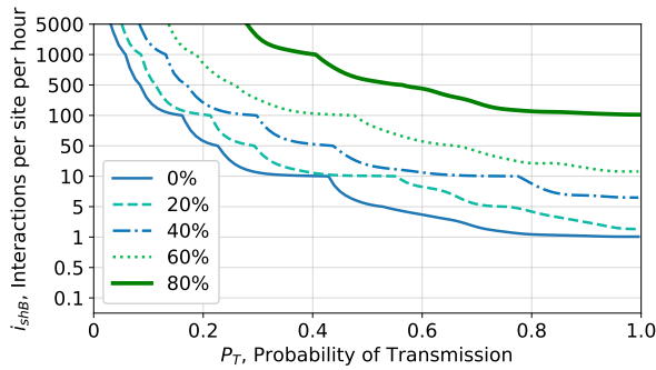
Fig. 7: Epidemic thresholds as different fractions of the population are vaccinated as a function of probability of transmission, P_T , and number of interactions per site per hour, i_{sh,B} .
