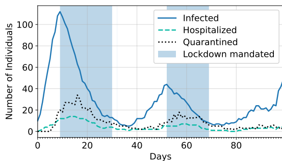
Fig. 3: Sample of a simulation with masking and testing always mandated, where the lockdown is triggered when 1% of the current population is showing infection symptoms and is turned off when below 0.1%.
