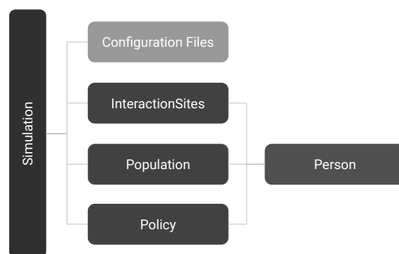
Fig. 1: Software framework used for mathematically modelling COVID-19 with QUABOOM, in Kingston, Ontario, Canada. Each dark box corresponds to a class in the code which can be configured through a set of configuration files in TOML format.
