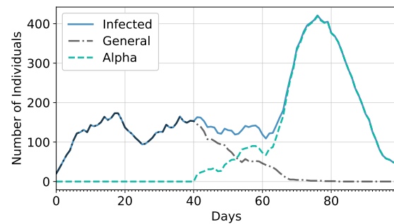
Fig. 4: Sample of a simulation with a lockdown, masking and testing always mandated, where a more infectious variant, called alpha, is introduced on day 40. The alpha variant is set to be 1.8 more contagious than the original variant.
