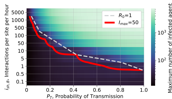
Fig. 6: A two-dimensional plot of mean max infected, I_{\max} (logarithmic colour scale), as a function of the probability of transmission, P_T , and the average number of interactions in level B sites per hour per site, i_{sh,B} , (logarithmic) in a population of N = 10\,000 . The dashed white line corresponds to defining an epidemic threshold based on \mathcal{R}_0 \geq 1 . The solid red line shows that an equivalent and smoother threshold can be defined with the value I_{\max} = 50 in this particular configuration of simulations.
