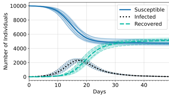
Fig. 2: Output of epidemic with a population size of 10000, a masking probability of 0.8, an attendance probability of 2/7 and a probability of transmission of 0.25. Each compartment (Susceptible, Infected, and Recovered) has a superposition of 5 runs (faded lines), the average of all the runs (in a thick line), and a 95% confidence interval (in the shaded region).
