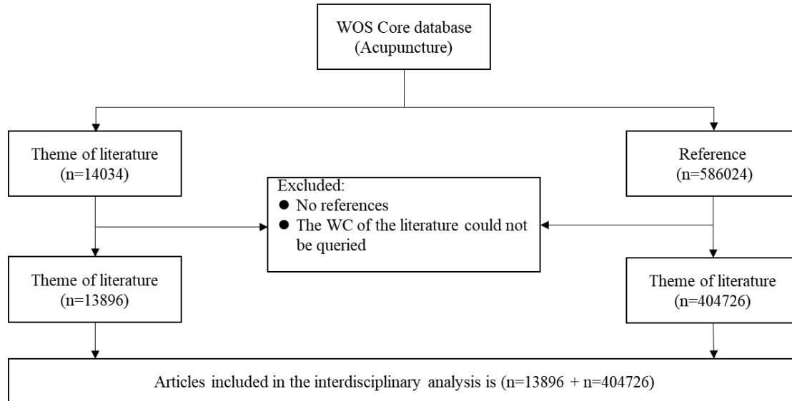
Fig. 1 Retrieval Flowchart
