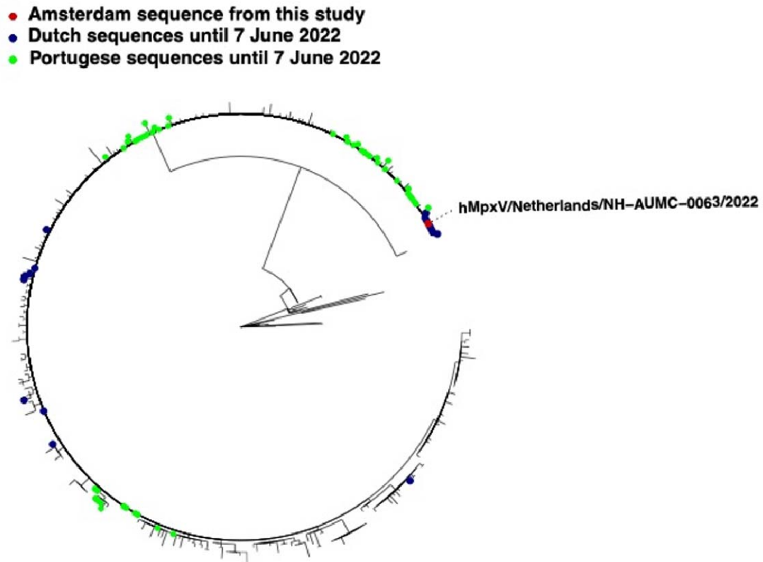
Figure 1: Phylogenetic association of one human Monkey Pox Virus strain found in a sample from a visitor at the Amsterdam Centre for Sexual Health in the first week of May (week 18), 2022 (red), and 11 Dutch (blue) and 48 Portuguese (green) reference strains.
