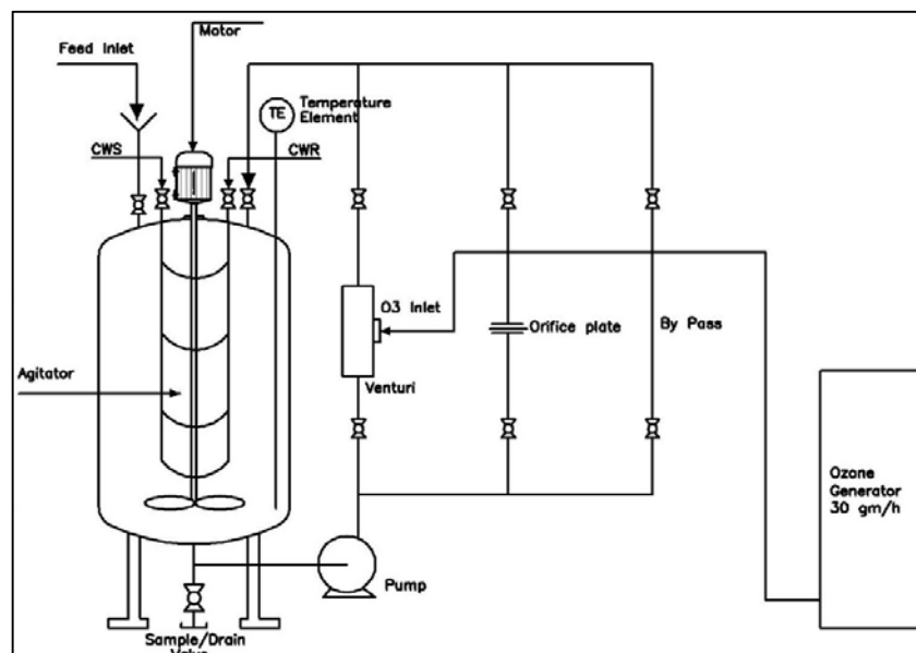
Fig. 2. Setup for hydrodynamic cavitation and its hybrid techniques.
