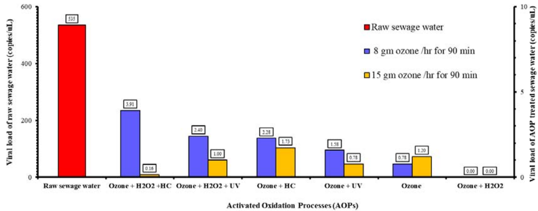
525 Fig. 5. Variations of initially screened treatment techniques using raw sewage 526 water samples. The Y-axis at the left shows the viral load (copies/μL) of raw sewage 527 water (red bar), and the secondary Y-axis axis depicts the viral load (copies/μL) of AOP 528 treated sewage water.
