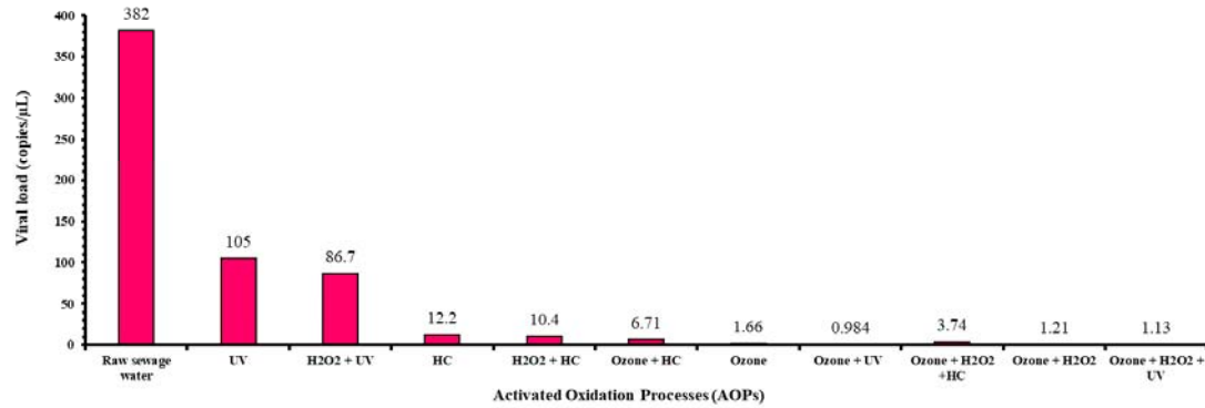
522 Fig. 4. Bar plot illustrating evaluation of disinfecting efficiency of different AOPs 523 for reduced viral load.
