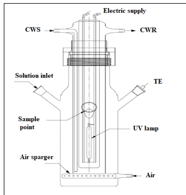
Fig. 3. Setup for UV/ozonation and its hybrid processes.
