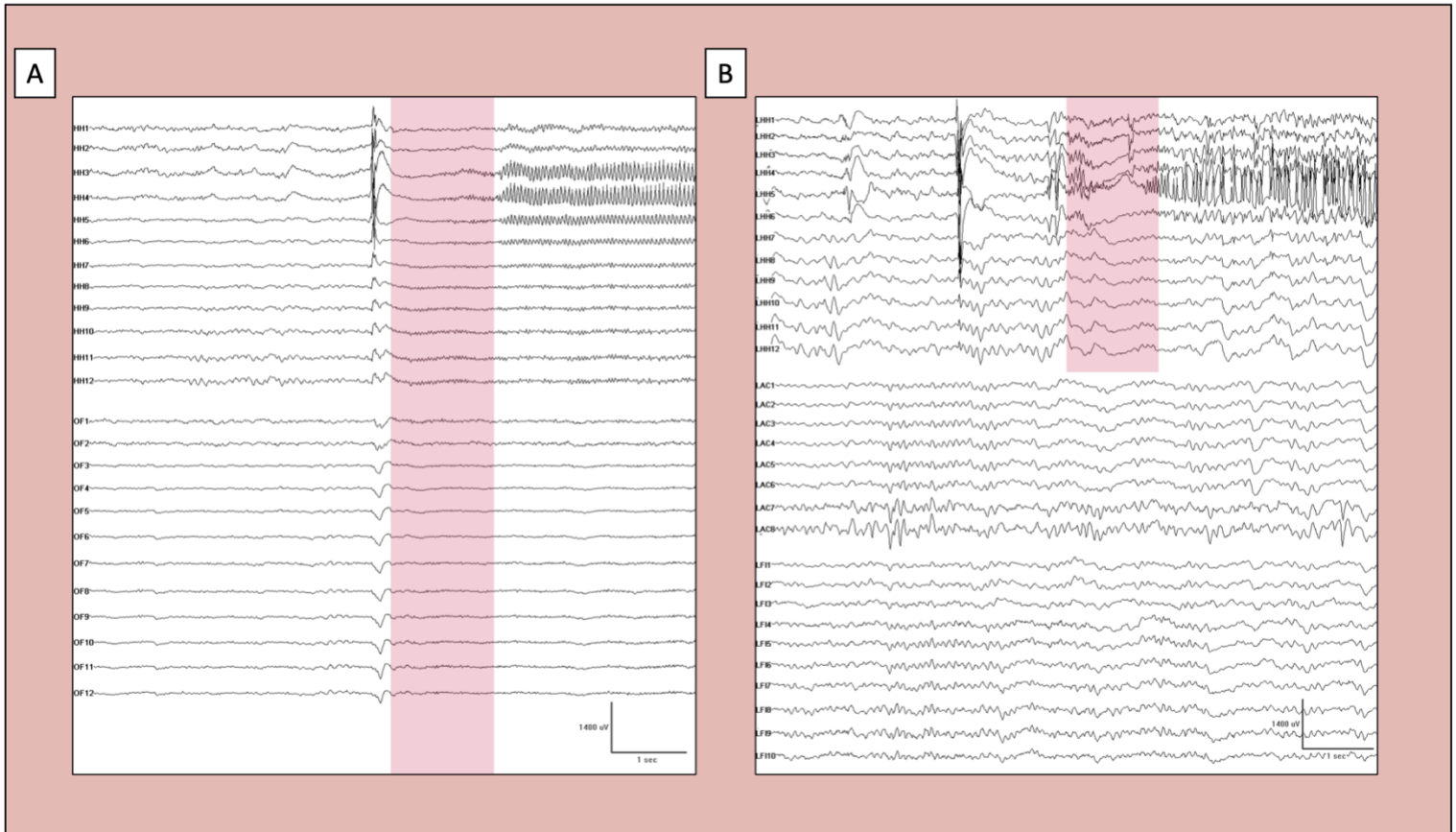
Figure 2. Electrodecrement (shaded areas). A. Diffuse electrodecrement which manifests as attenuation with or without superimposed faster frequencies at the site of seizure onset (hippocampal head; HH) as well as the lateral contacts and more distant contacts that were not primarily involved with the seizure (orbitofrontal cortex; OF). B. Focal electrodecrement constrained to the site of seizure onset (hippocampal head—LHH) but not prominently in the lateral or extratemporal contacts. Note the ongoing oscillatory activity in the anterior cingulate (LAC) and frontal to insular (LFI) contacts.
