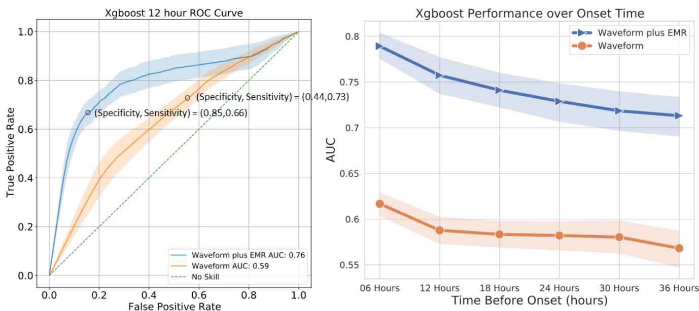
Figure 2. Receiver Operating Curve for 12 Hour Model (left) and Trajectory of Models as Prediction Horizon Approaches Onset
