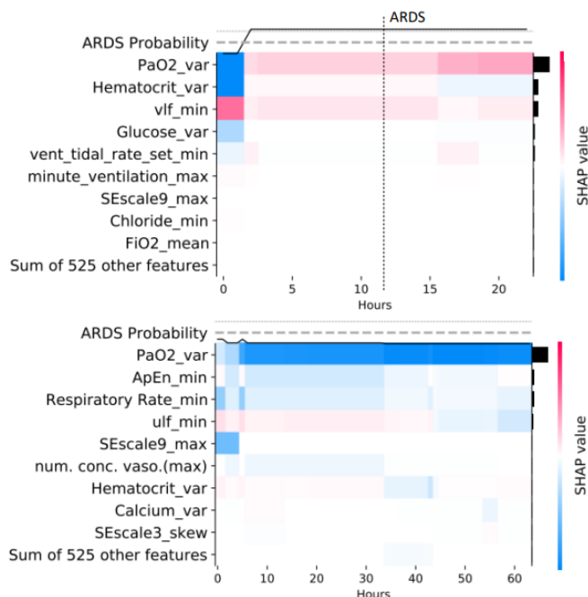
Figure 4. Case and Control Patient Model Probability Trajectories and Associated SHAP Values
