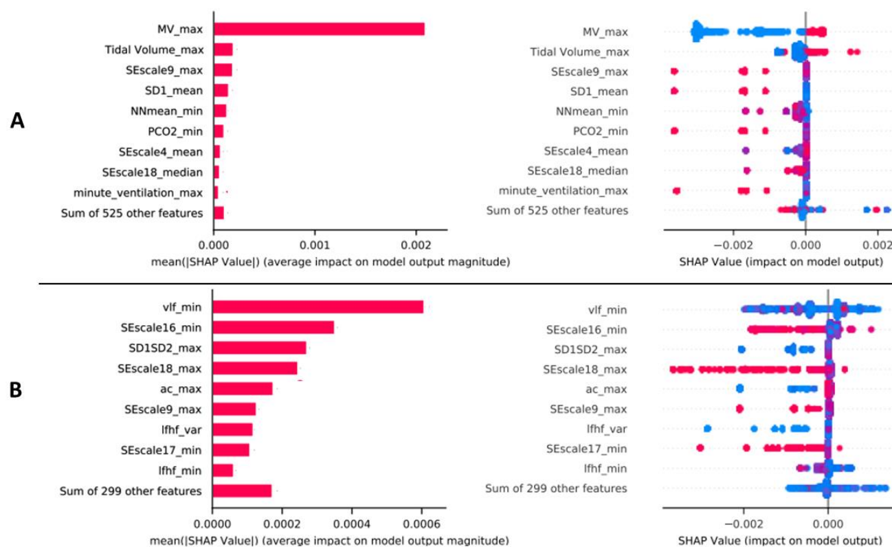
Figure 3. SHAP Magnitude and Beeswarm Plot for Combined Features (A) and Waveform-only Features (B) Models
