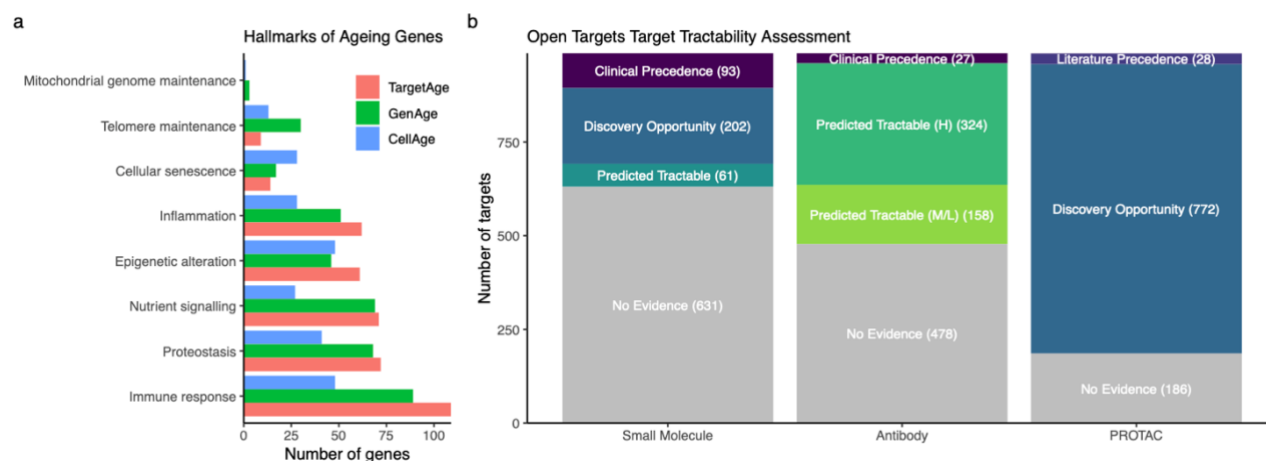
Fig 3) a) The proportion of genes annotated with at least one GO term corresponding to each Hallmarks of Ageing category, for the TargetAge gene set (red), GenAge (green) and CellAge (blue). b) Tractability categorisations when considering Small Molecule, Antibody, or PROTAC therapeutic approaches. Categorisations are based on the existence of an approved or experimental drug (Clinical Precedence), literature reports for PROTAC (Literature Precedence), and different levels of experimental and computational evidence.
