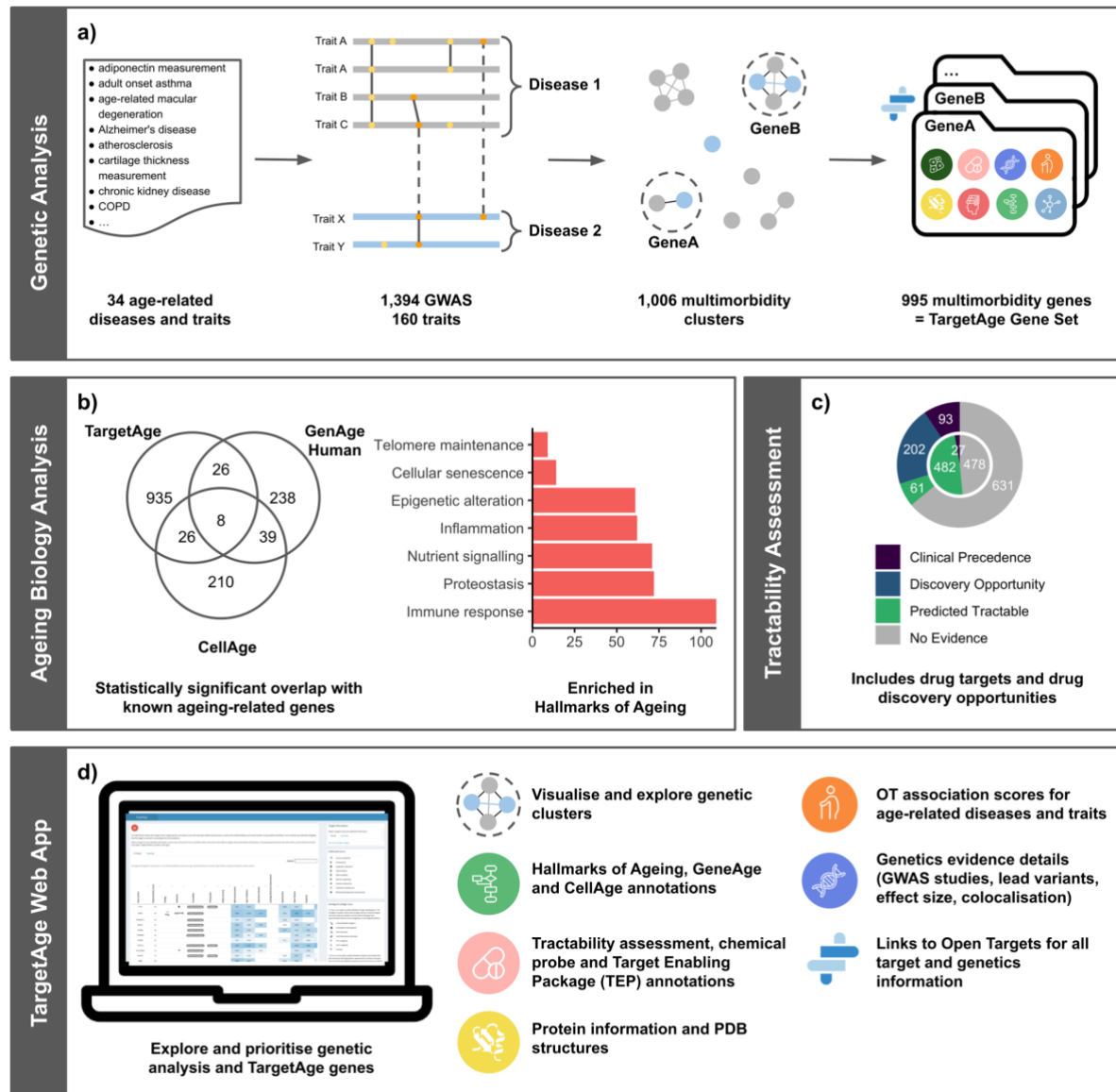
Figure 1) Overview of the TargetAge analysis. a) Genetic Analysis: GWAS data from Open Targets Genetics is retrieved for 34 age-related diseases and traits and descendant terms in the Experimental Factor Ontology (EFO). Overlapping genetic hits that may share a causal variant are clustered to identify independent genetic signals. Clusters containing multiple age-related diseases are mapped to candidate causal genes using the L2G method from Open Targets Genetics. Target annotations are retrieved from Open Targets Platform for the 995 resulting protein coding genes, referred to as the TargetAge gene set. b) Ageing Biology Analysis: The TargetAge set has statistically significant overlaps with three sets of age-related genes: GenAge, CellAge, and genes annotated with GO terms mapped to the Hallmarks of Ageing. c) Tractability Assessment: The TargetAge set were assessed for clinical precedence and tractability as drug targets using a therapeutic antibody (outer ring) or small molecule (inner) approach, as well as for the availability of chemical probes and Target Enabling Packages (TEPs). d) TargetAge Web App: The TargetAge gene set are presented in a freely available web application including the genetic evidence, target annotations, links to ageing, and tractability assessment.
