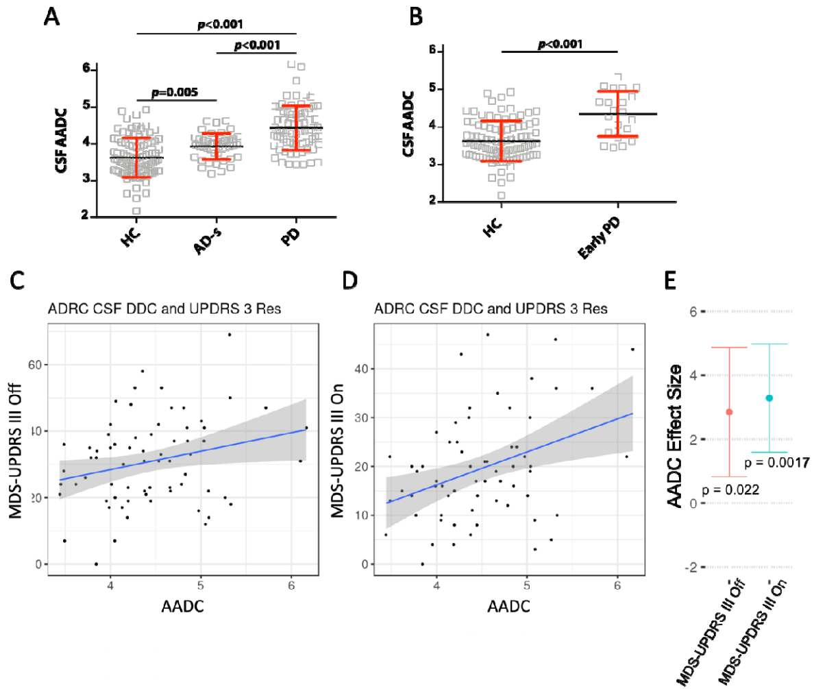
Figure 2. A.) CSF AADC levels are elevated in AD and PD participants, with greater elevation in PD. Test statistics from Wilcoxon Rank Sum test. B.) AADC levels are elevated in early PD participants. Test statistics from Wilcoxon Rank Sum test. C.) CSF AADC levels are associated with clinician-assessed motor symptom severity in Parkinson's disease participants as measured by the MDS-UPDRS III Off score. D.) CSF AADC levels are associated with clinician-assessed motor symptom severity in Parkinson's disease participants as measured by the MDS-UPDRS III On score. E.) Effect size and significance for relationships in C,D.
