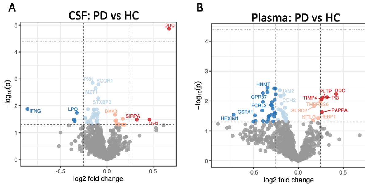
Extended data figure 6. Differential expression analysis of Parkinson's disease participants in the PPMI cohort using all longitudinal samples. Differential expression is performed with a multi-level mixed effects model controlled for age, sex, demographics, and sample-relatedness. Lower horizontal dotted line indicates FDR significance threshold, upper horizontal line indicates Bonferroni significance threshold. Dotted vertical lines indicate an arbitrary 0.25 \log_2 fold change cutoff for differential expression. Significant hits are colored and
