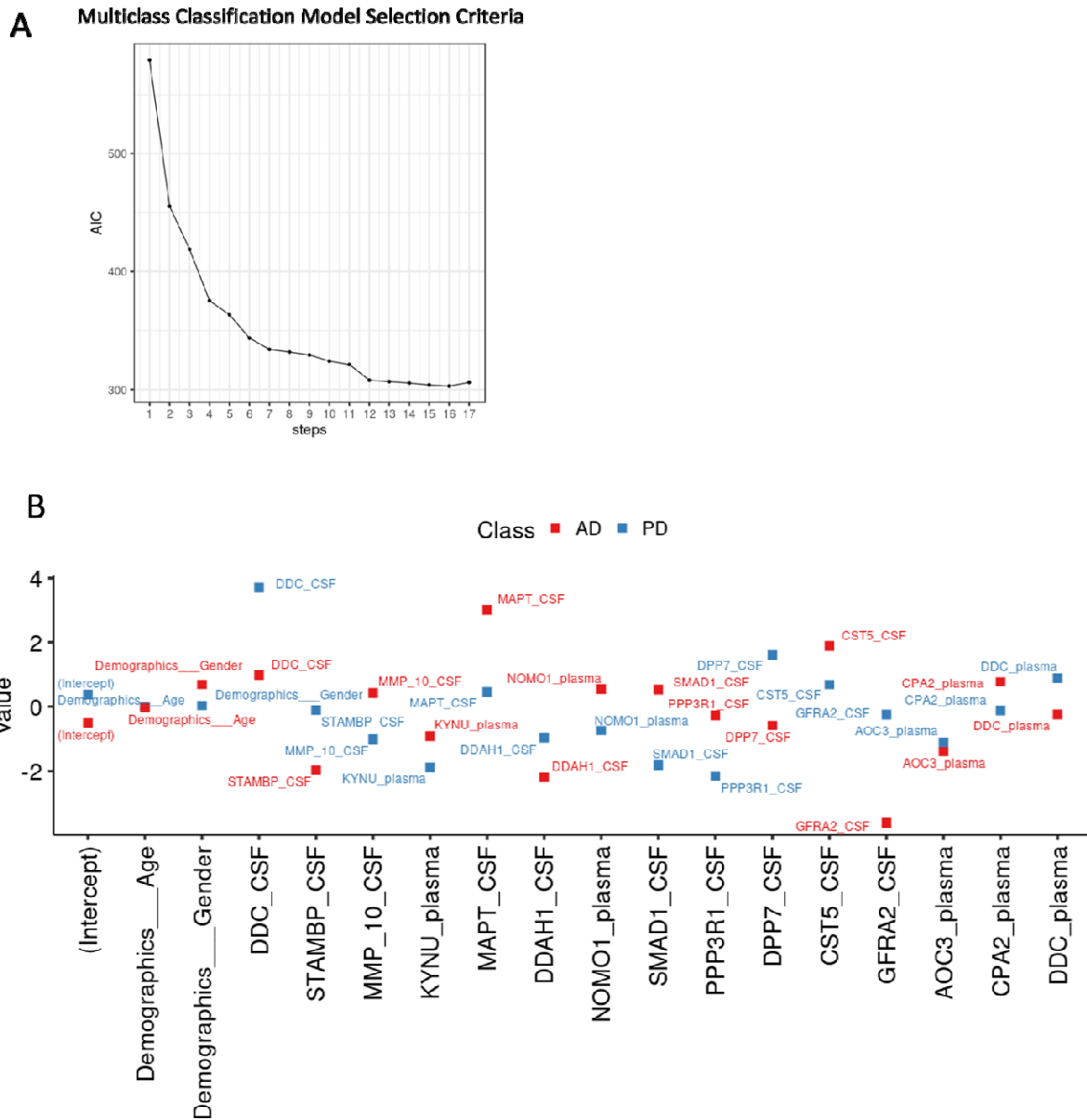
Extended data figure 9. A stepwise multi-class logistic regression was run using the top 15 hits from differential expression of PD vs AD and PD vs HC participants, in both CSF and plasma. A model was built up by iteratively testing the addition of one additional biomarker to previous model (one step) and evaluating the Akaike Information Criteria (AIC) for all possible stepwise combinations. The baseline model included DDC in CSF, age, and gender (step 1). A) The optimal model based on AIC had 15 additional biomarkers, before the AIC began to increase and the model performed sub-optimally. B) Feature weights for the combined biomarker PD classification model trained with L2 penalized logistic regression. Proteins are shown in order of model inclusion using stepwise forward logistic regression.
