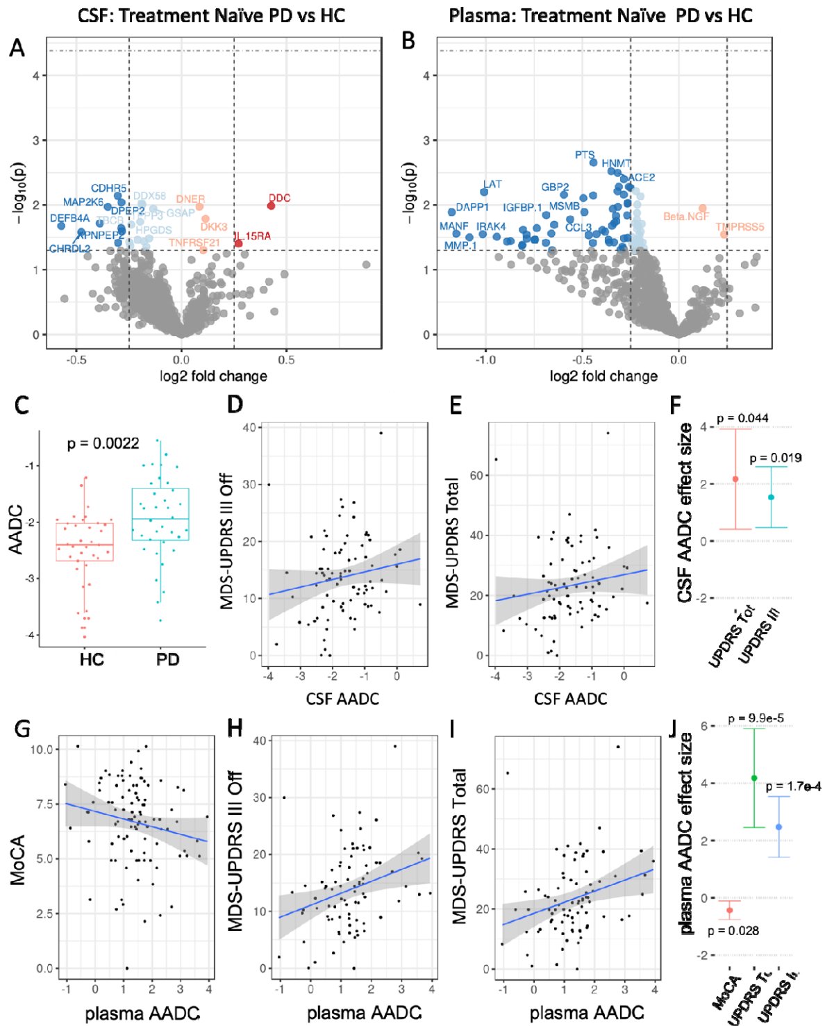
Figure 3: Replication of AADC findings in an independent treatment naive Parkinson's Disease population. A,B.) CSF (A) and plasma (B) differential expression analysis of treatment naive Parkinson's participants at baseline compared to healthy control participants at baseline. Linear modeling controlled for age, sex, and demographics. P values are shown instead of FDR-corrected p values. Due to small sample size of the cohort, no
