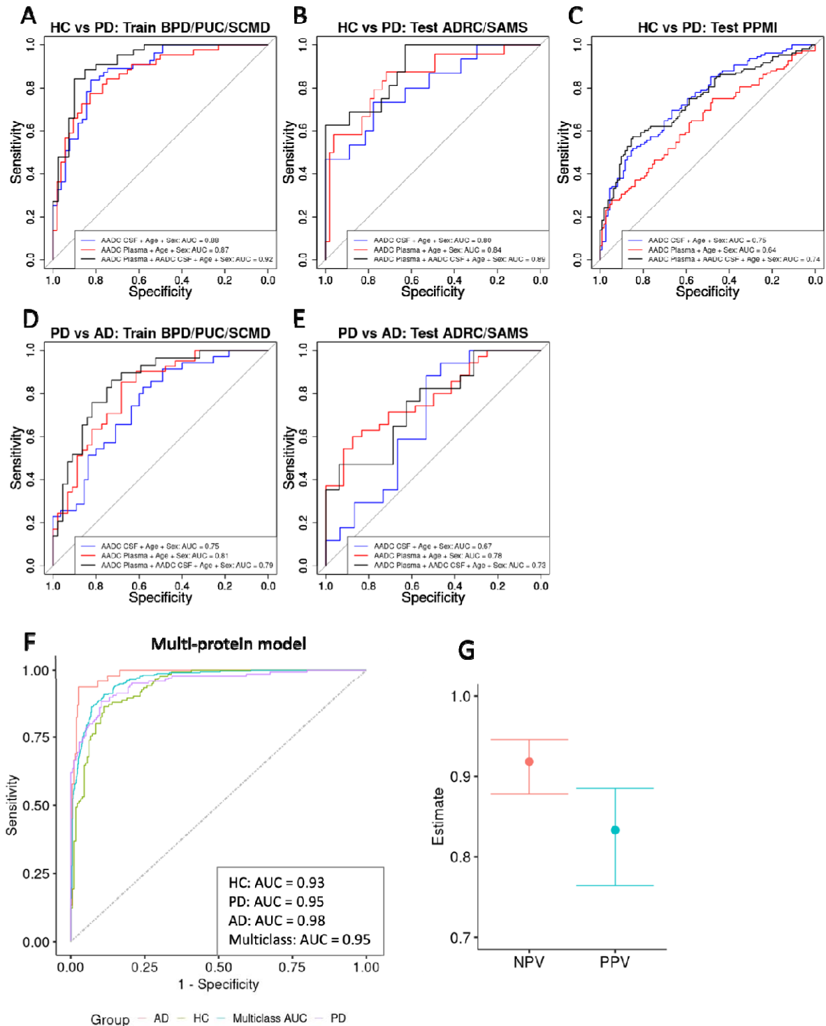
Figure 4. Development and testing of logistic regression classifiers to discriminate PD participants from healthy controls and AD participants using AADC levels in CSF and plasma. Receiver operating characteristic (ROC) sensitivity-specificity curves of classifier performance are plotted. Area Under the Curve (AUC) is a measure of classifier performance, with an AUC of 1 being perfect classification with no false positives (perfect specificity)
