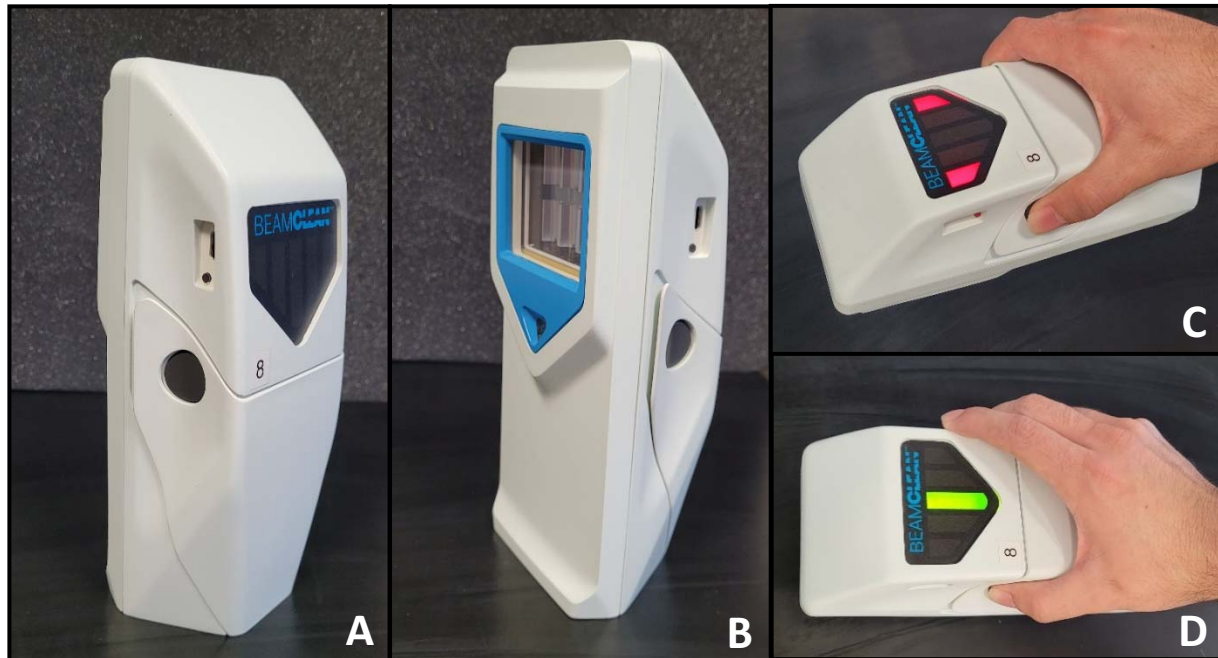
Figure 1. The portable battery-operated FFUV handheld disinfection device A) side view showing the “on” button (round black) on the device that needs to be held down during operation B) side view of the device showing the glass surface area in the bottom that emanates the UV-C light C) The “red indicator light” suggests the correct distance for the surface to be disinfected has been not yet achieved. D) The “green indicator light” indicates the correct distance has been reached.
