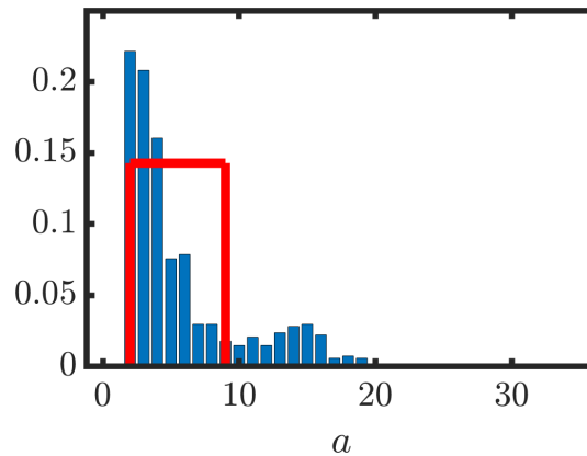
Figure 1: The age (days) distribution, f , of supplied units at a Scottish District hospital (blue bars). Red line denotes approximated uniform distribution (see equation (2.15)). Data provided by Scottish National Blood Transfusion Service.
