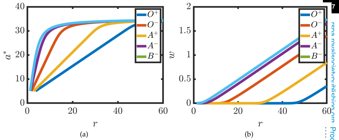
Figure 4: Exploring the effect of varying the restock threshold, r . (a) The minimum age of transfused units, a^* , is plotted against r (see equation (2.41)). (b) Wastage rate, w , is plotted against restock threshold, r , (equation (2.33)). Parameter values (for Time period 1) as in Tables 2 and 3 unless otherwise stated. Note that B^+ , AB^+ and AB^- were not stocked.
