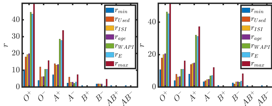
Figure 6: A summary of different estimates for restock thresholds for the different blood groups. (a) Time period 1. (b) Time period 2. Parameter values as in Tables 2 and 3. T_{W API} = 0.2 , T_{age} = 16 .
