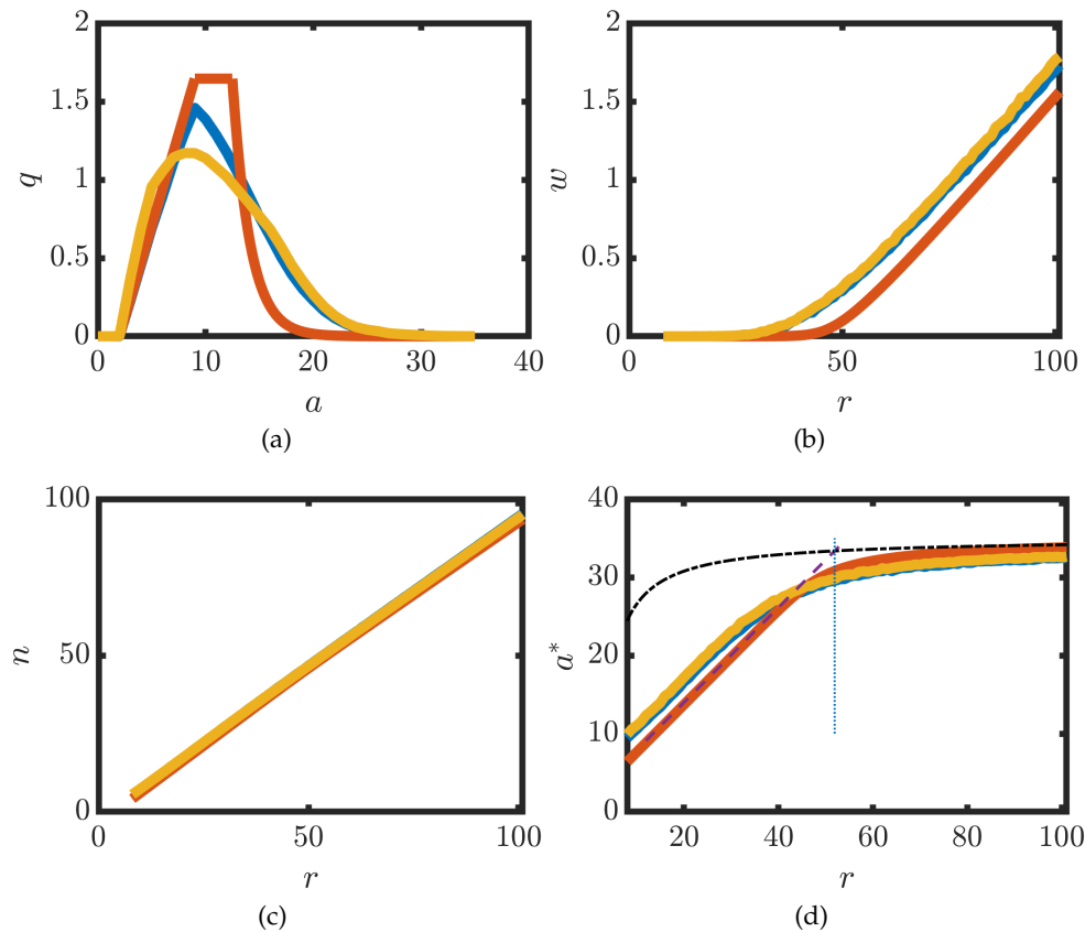
Figure 2: Comparison of key mode outputs. (a) Number density, q , is plotted against age, a . r = 18 . (b) The wastage rate, w , is plotted against restock threshold, r . (c) Total stock, n , is plotted against restock threshold, r . (d) Minimum age of transfused units, a^* , is plotted against restock threshold, r . Blue lines - time average of discrete model with uniformly distributed age supply pdf. Yellow lines - time average of discrete model with empirically estimated age supply pdf. Red lines - continuum model. Continuum model solutions for q , w , n and a^* given by equations (2.20), (2.33), (2.22) and (2.25), respectively. Asymptotes in (d) given by equations (2.27) and (2.28). Dotted vertical lines represent onset of waste (equation (2.30)). k_2 = 1.57 . \tau = 0 . Discrete model given by equations (2.1)-(2.5). Other parameters as in Table 3.
