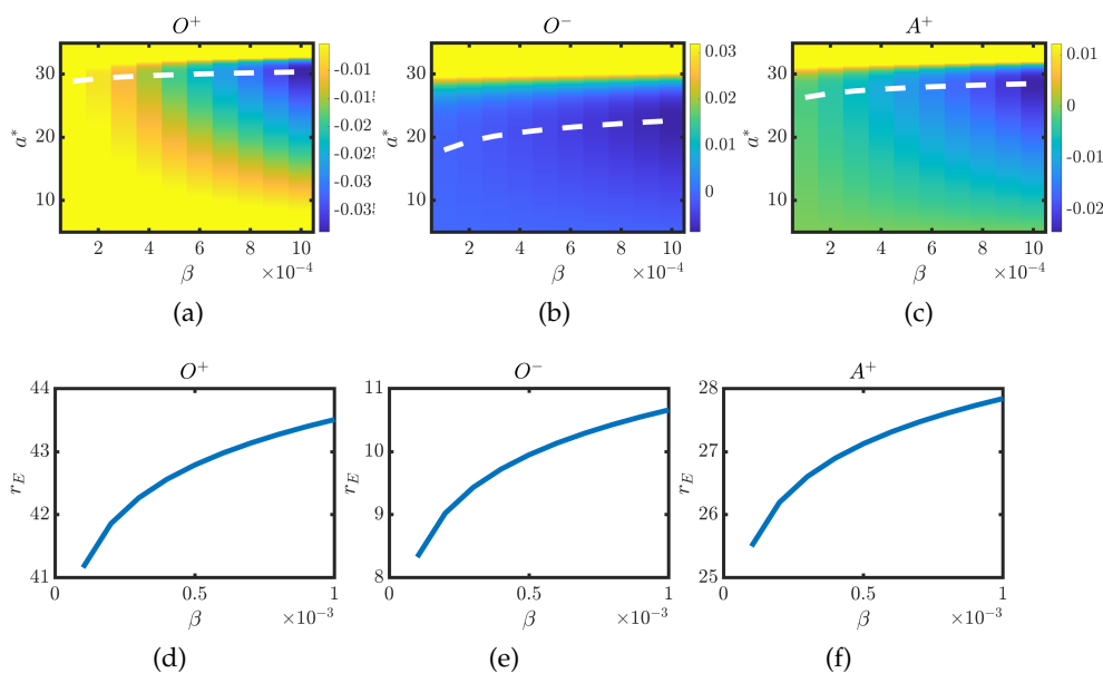
Figure 5: Optimal restock thresholds for selected blood groups. (a-c) The value of the objective function, E , (see equation (2.48)) is plotted against, a^* , and \beta . Colour represents E and the dashed lines local minima. (d-f) Optimal solution, r_E , is plotted against weighting parameter, \beta ( r_E is computed by numerically finding a^* that minimises E and then using equation (2.26)). Parameter values as in Tables 2 and 3 unless otherwise stated.
