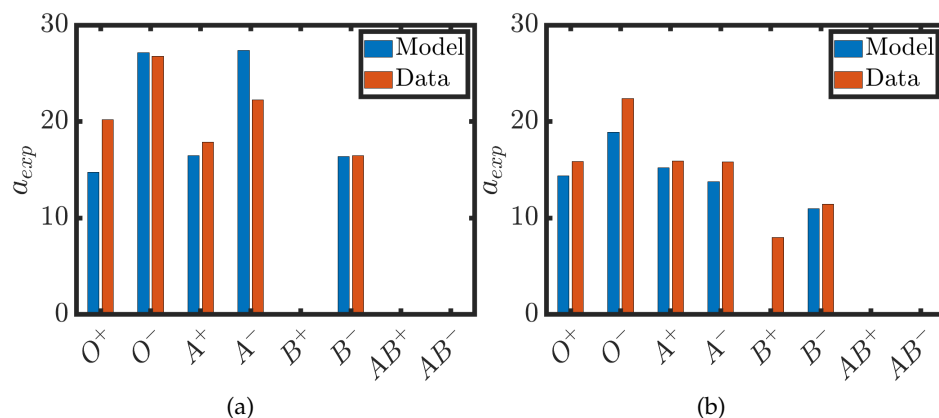
Figure 3: Expected age of transfused units, a_{exp} , is plotted for different blood groups. (equation (2.41)). (a) Restock threshold for time period 1. (b) Restock thresholds for time period 2. Model data (blue bars) generated using equation (2.41). See Tables 2 and Table 3 for parameter values.
