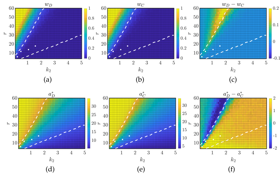
Figure 7: Comparison of discrete and continuum model outputs. Wastage rate, w_D , in the discrete model is plotted against restock threshold, r , and demand rate, k_2 . (b) The corresponding wastage rate in the continuum model, w_C . (c) The difference between wastage rates in the discrete and continuum models ( w_D - w_C ). (d) The minimum age of transfused units in the discrete model, a_D^* , is plotted against restock threshold, r , and demand rate, k_2 . The corresponding minimum age of transfused units in the continuum model, a_C^* . (f) The difference between minimum age of transfused units in the discrete and continuum models ( a_D^* - a_C^* ). Dashed lines represent contours a^* = a_1 and a^* = 30 . White dots represent parameters used for different blood groups at the Scottish DGH under study (see Table 2). Continuum model solutions for w and a^* given by equations (2.33) and (2.25), respectively. \tau = 0 . Discrete model given by equations (2.1)-(2.5). Other parameters as in Table 3.
